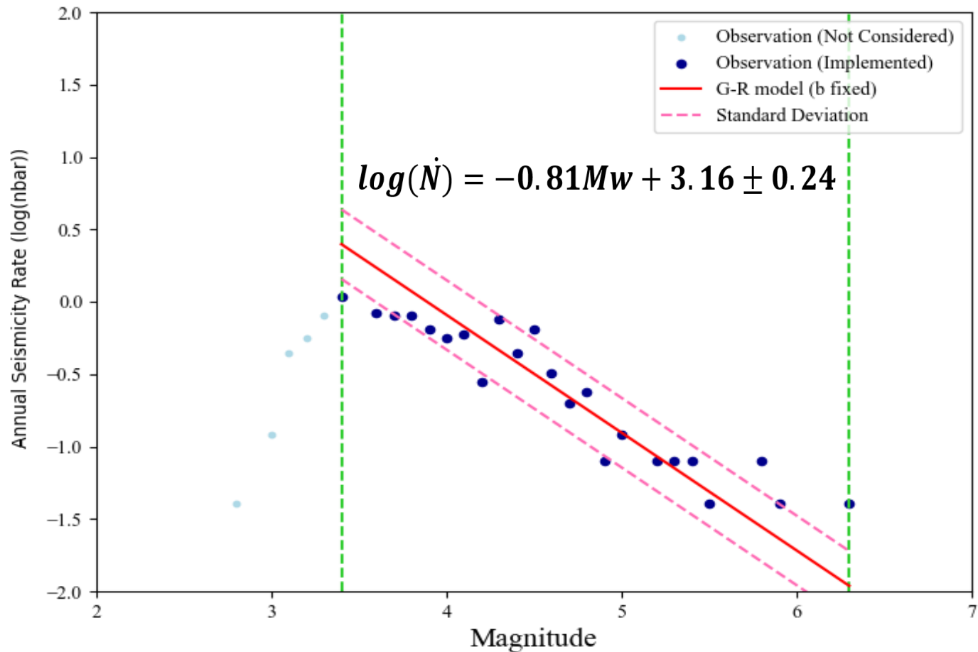
Magnitude–frequency distribution used for a-value estimation in Zone 10 (Grünthal pers. comm.)
