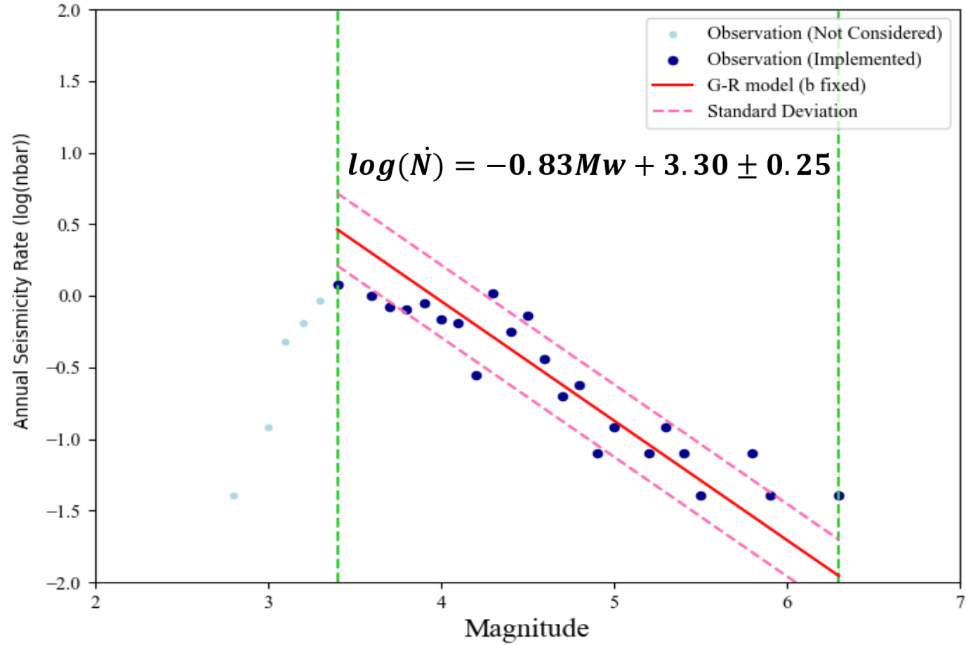
Magnitude–frequency distribution used for a-value estimation in Zone 10 (Gardner & Knopoff, 1974)
