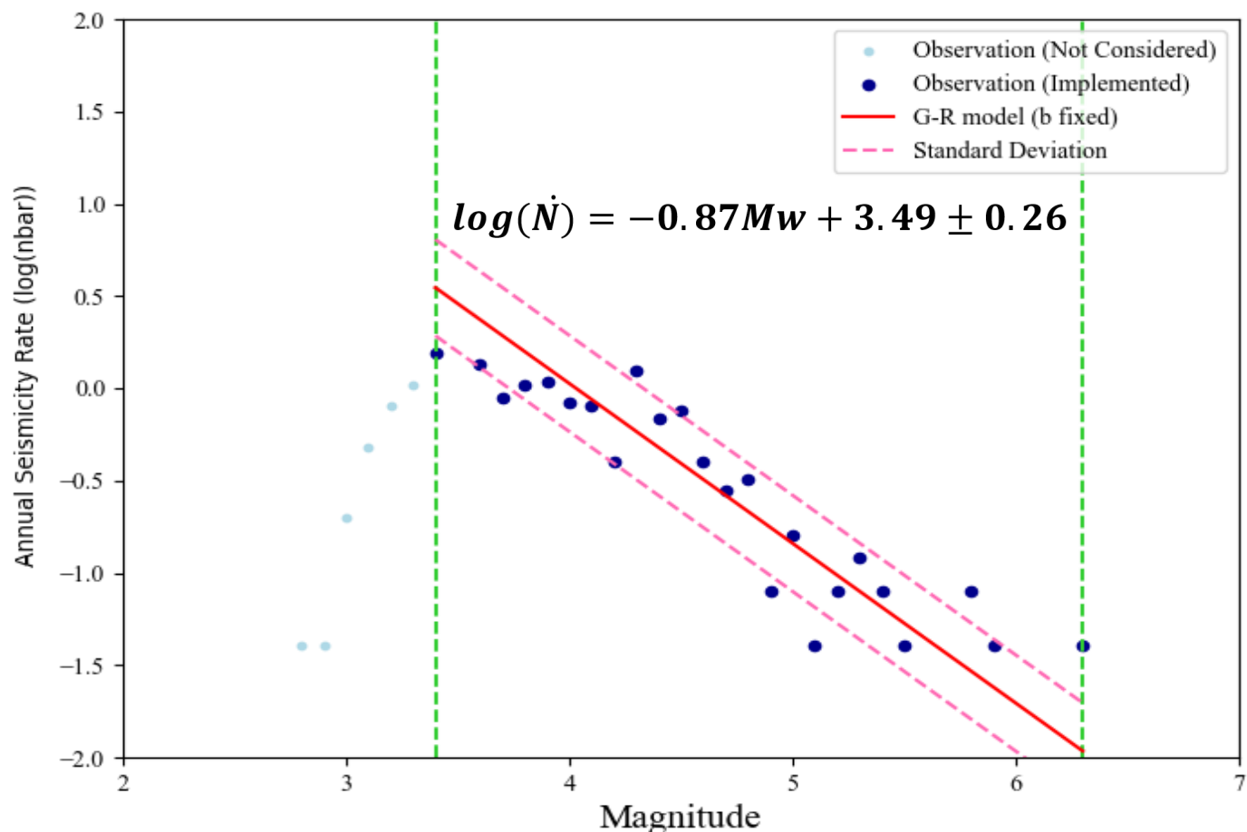
Magnitude–frequency distribution used for a-value estimation in Zone 10 (Uhrhammer, 1986)
