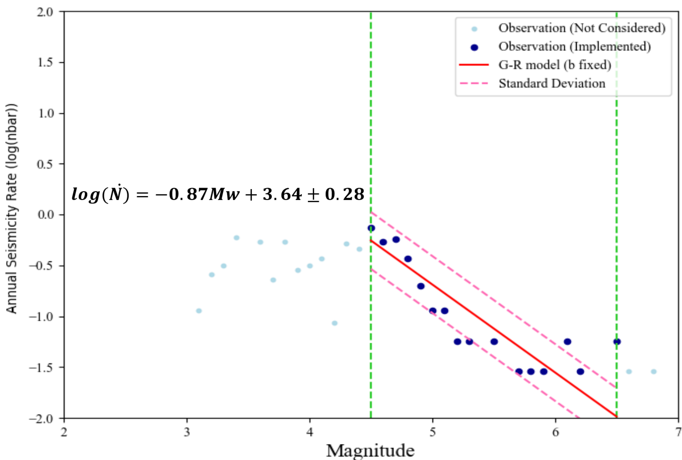
Magnitude–frequency distribution used for a-value estimation in Zone 12 (Uhrhammer, 1986)
