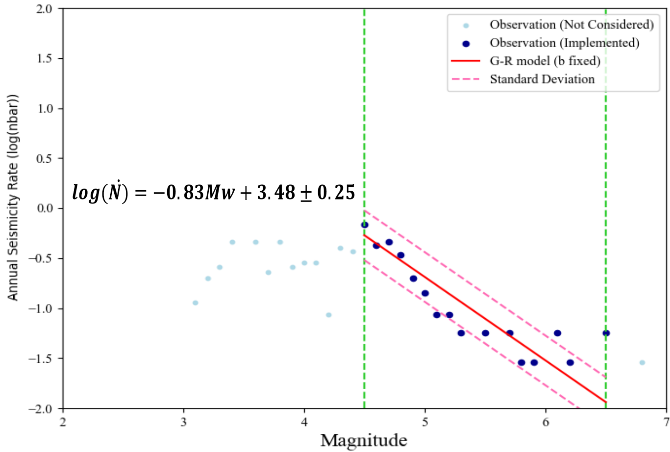
Magnitude–frequency distribution used for a-value estimation in Zone 12 (Gardner & Knopoff, 1974)
