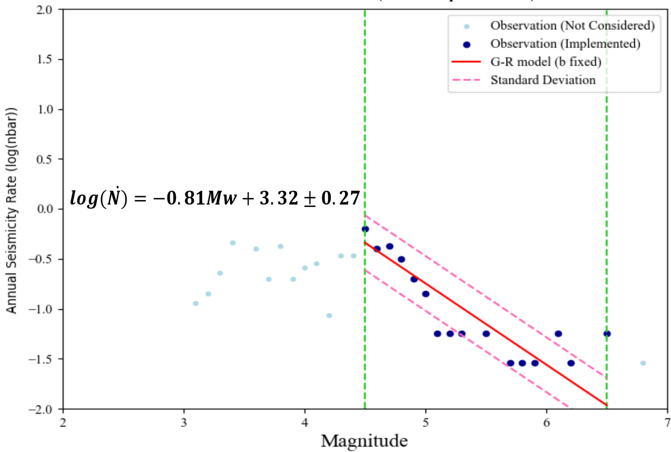
Magnitude–frequency distribution used for a-value estimation in Zone 12 (Grünthal pers. comm.)
