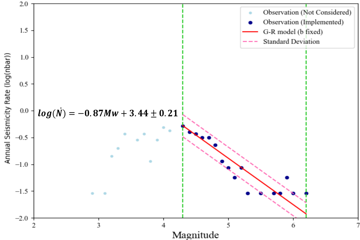
Magnitude–frequency distribution used for a-value estimation in Zone 13 (Uhrhammer, 1986)
