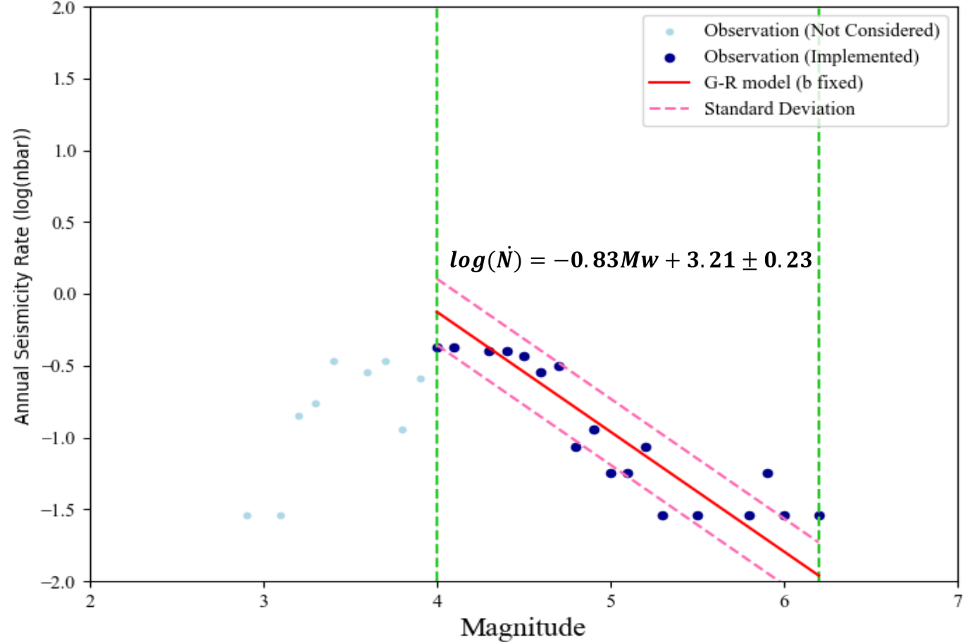
Magnitude–frequency distribution used for a-value estimation in Zone 13 (Gardner & Knopoff, 1974)
