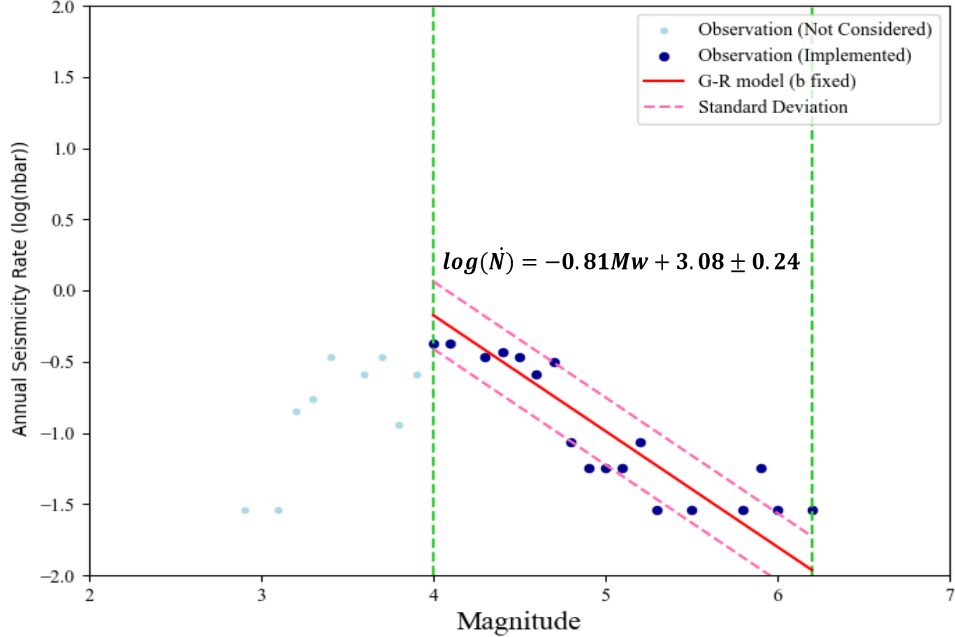
Magnitude–frequency distribution used for a-value estimation in Zone 13 (Grünthal pers. comm.)
