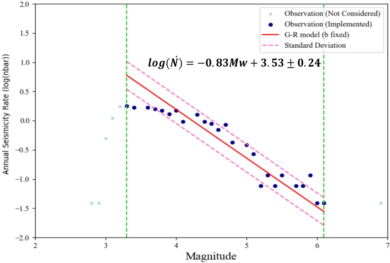
Magnitude–frequency distribution used for a-value estimation in Zone 14 (Gardner & Knopoff, 1974)
