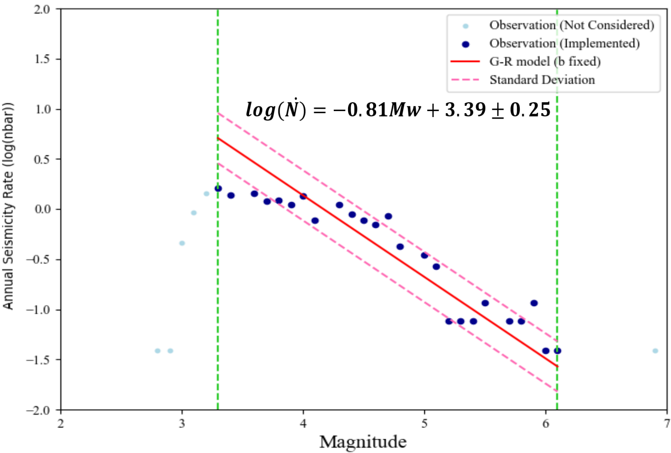
Magnitude–frequency distribution used for a-value estimation in Zone 14 (Grünthal pers. comm.)
