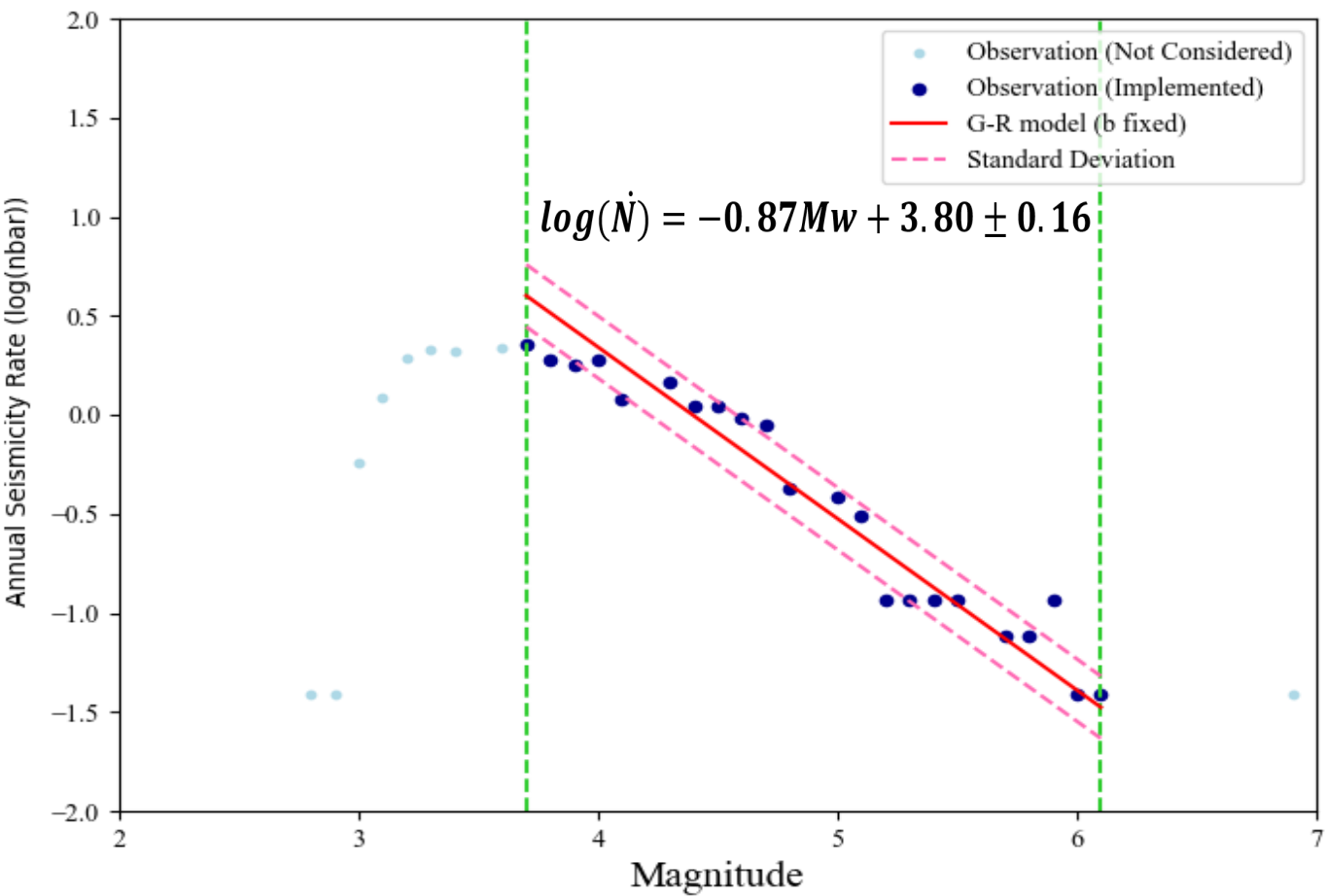
Magnitude–frequency distribution used for a-value estimation in Zone 14 (Uhrhammer, 1986)
