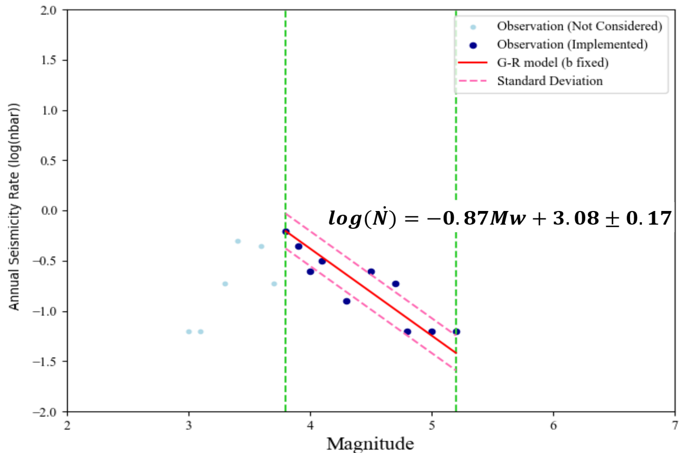
Magnitude–frequency distribution used for a-value estimation in Zone 16 (Uhrhammer, 1986)
