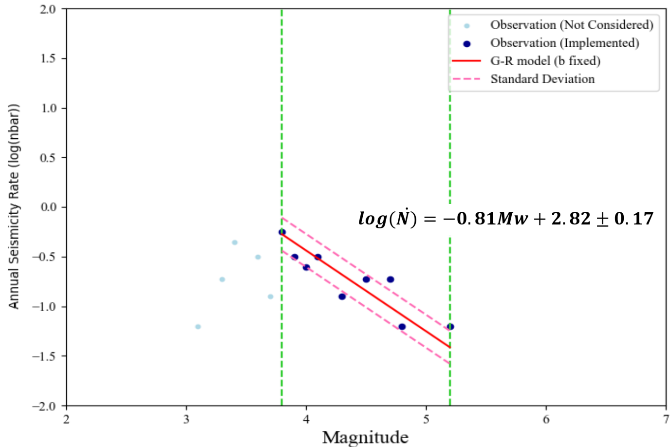
Magnitude–frequency distribution used for a-value estimation in Zone 16 (Grünthal pers. comm.)
