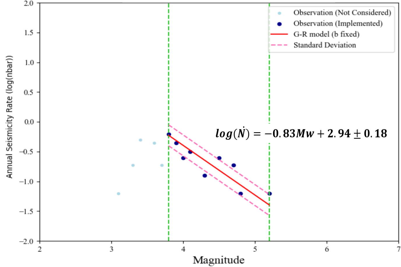
Magnitude–frequency distribution used for a-value estimation in Zone 16 (Gardner & Knopoff, 1974)
