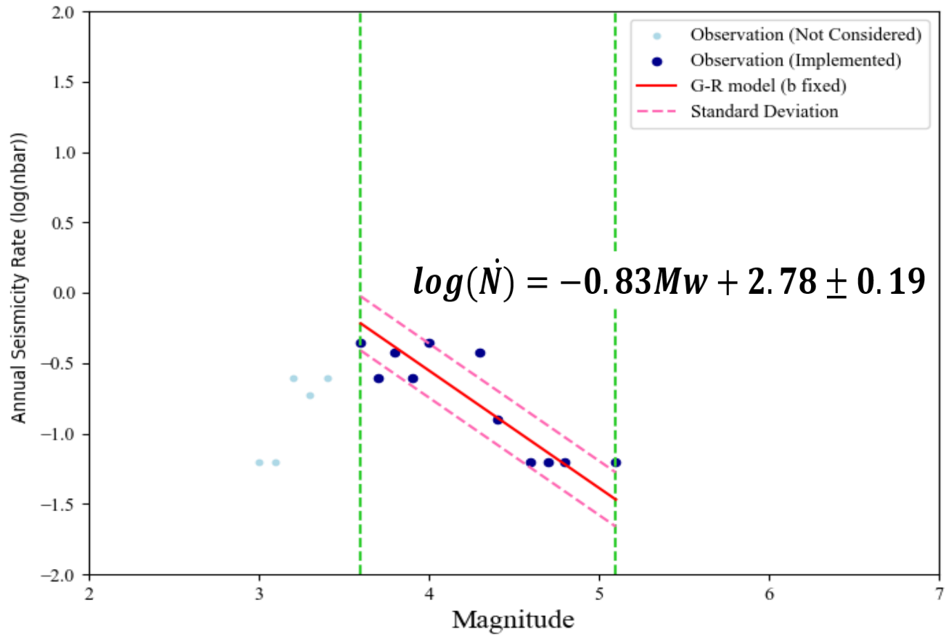
Magnitude–frequency distribution used for a-value estimation in Zone 18 (Gardner & Knopoff, 1974)
