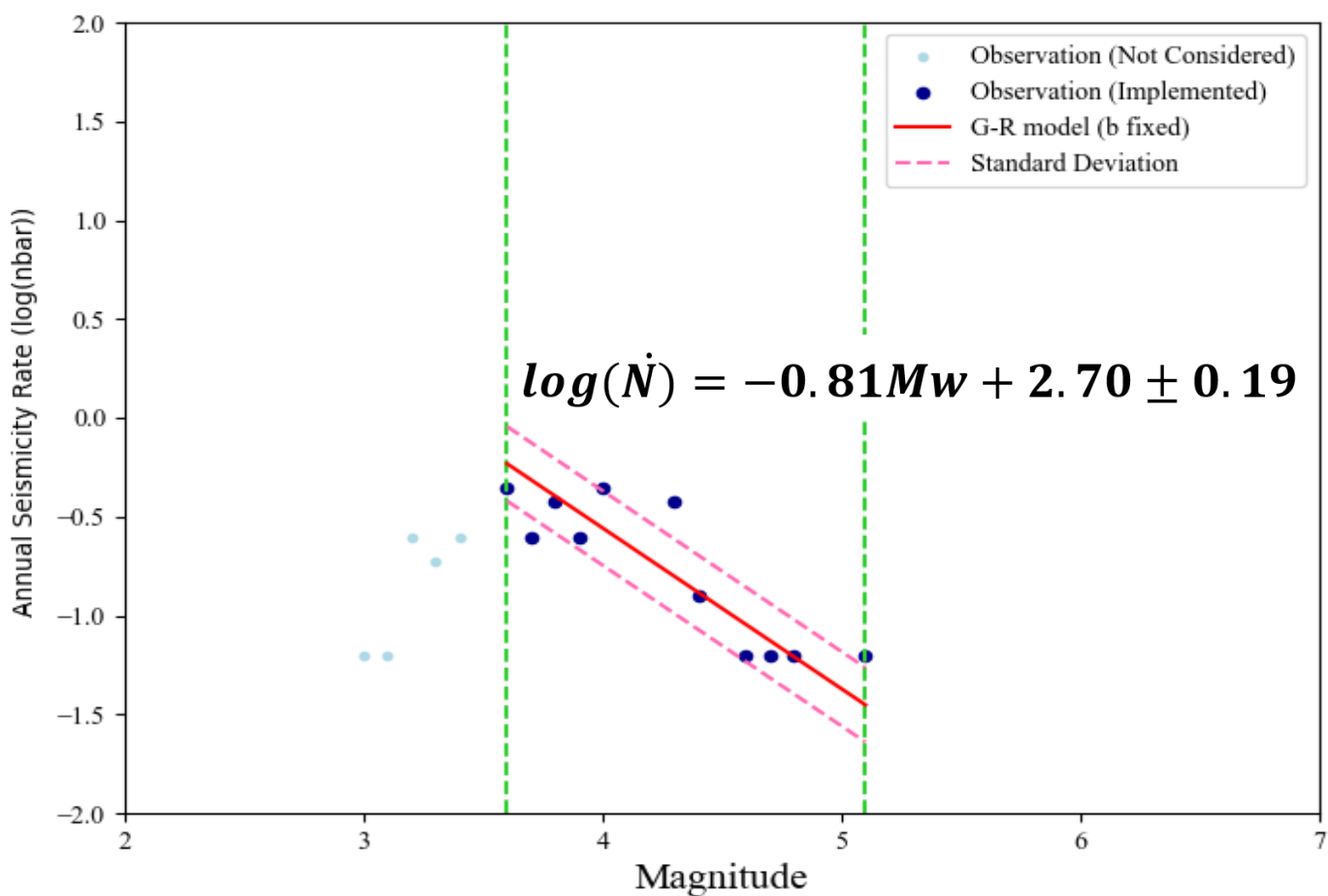
Magnitude–frequency distribution used for a-value estimation in Zone 18 (Grünthal pers. comm.)
