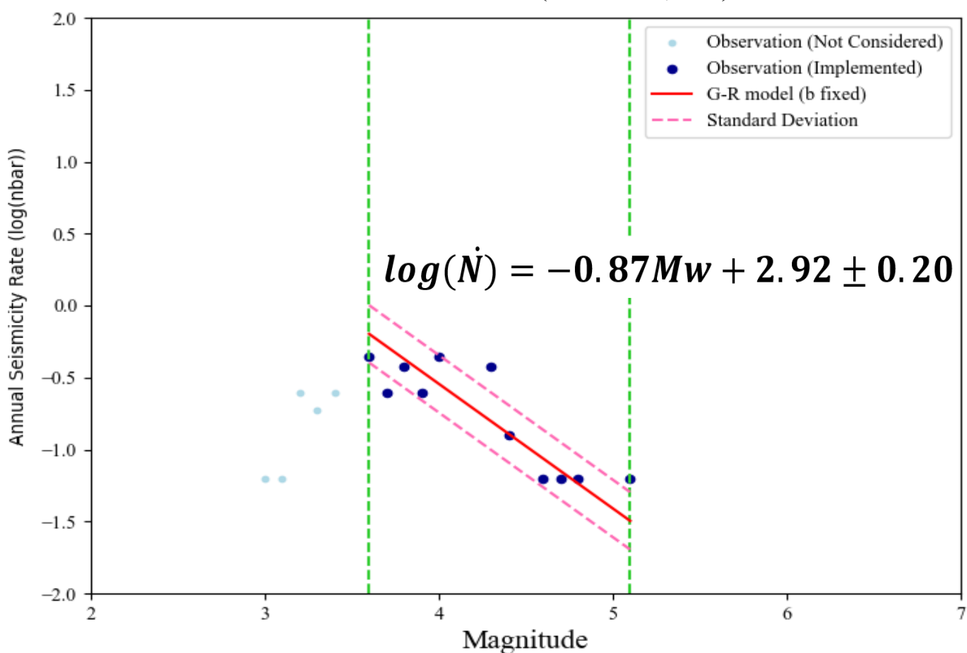
Magnitude–frequency distribution used for a-value estimation in Zone 18 (Uhrhammer, 1986)
