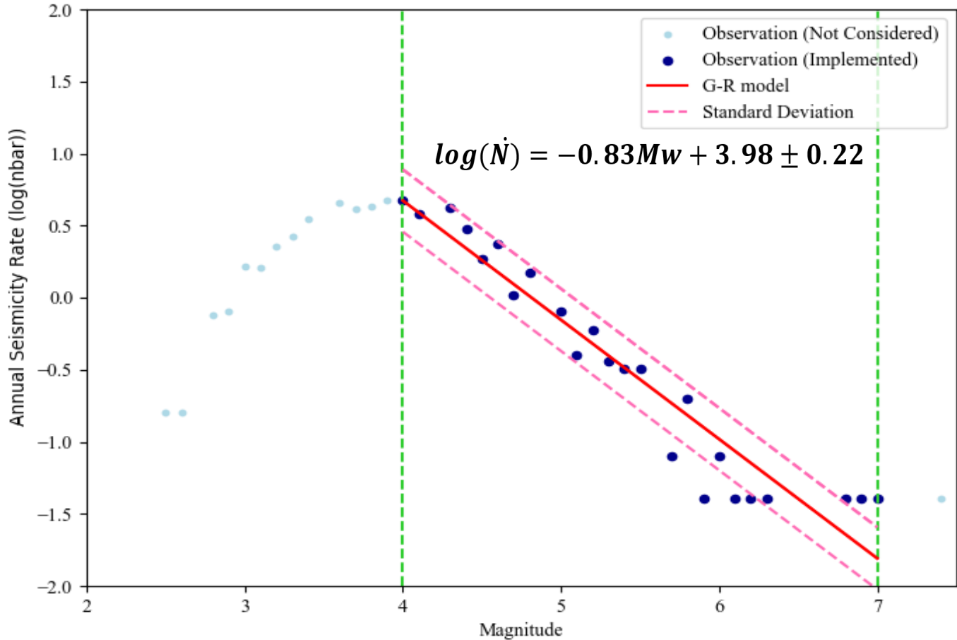
Magnitude–frequency distribution used for a-value and b-value estimation in Zone 18 (Gardner & Knopoff, 1974)
