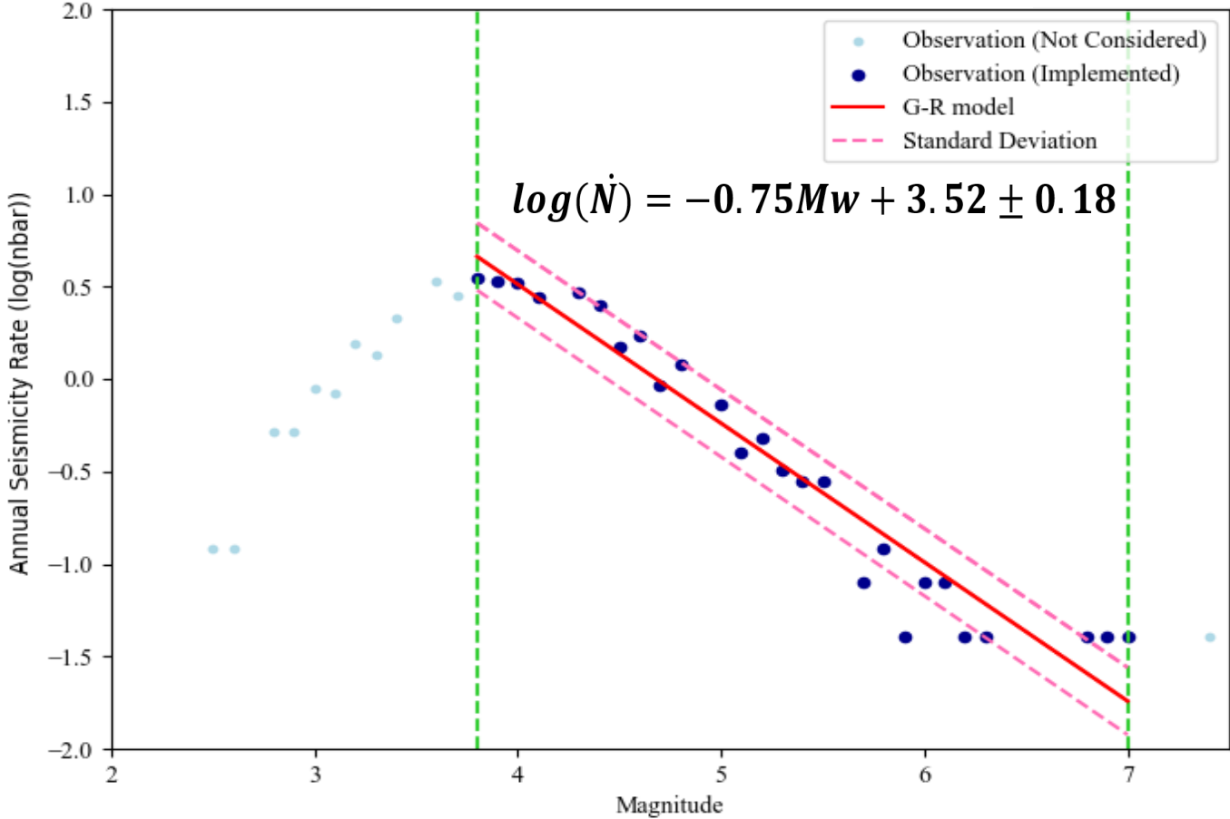
Magnitude–frequency distribution used for a-value and b-value estimation in Zone 18 (Grünthal pers. comm.)
