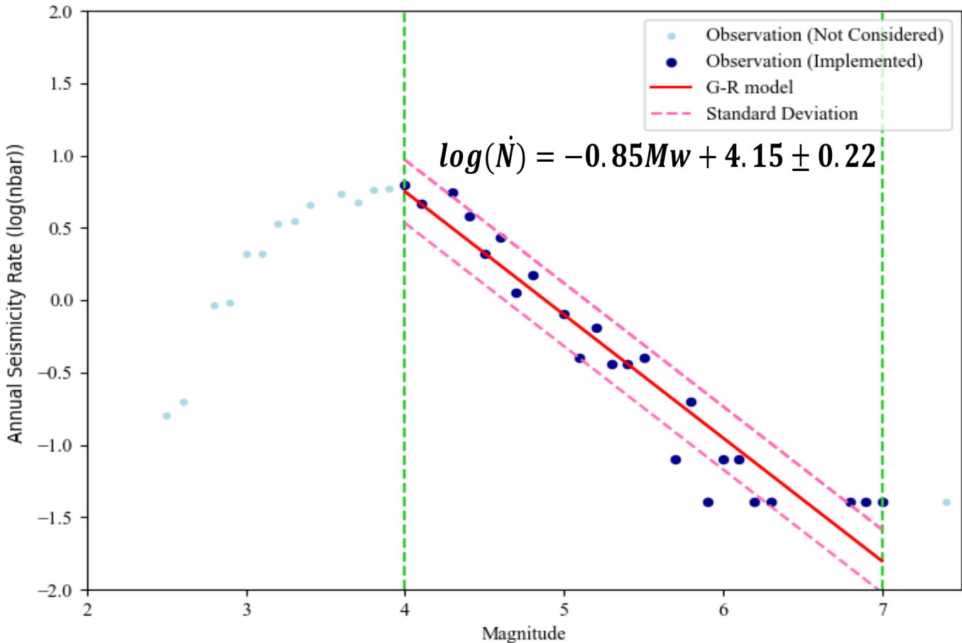
Magnitude–frequency distribution used for a-value and b-value estimation in Zone 18 (Uhrhammer, 1986)
