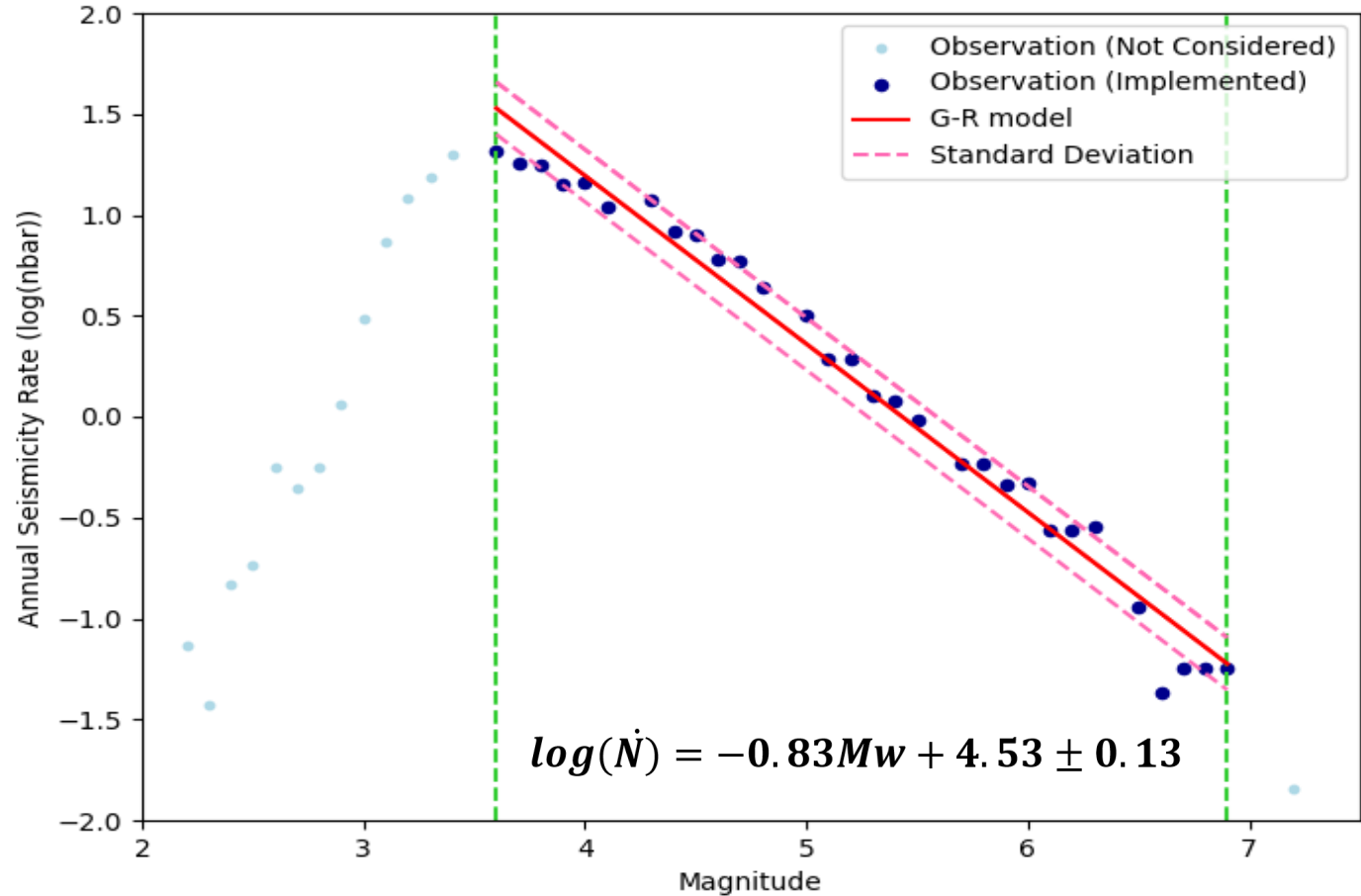
Magnitude–frequency distribution used for b-value estimation in the whole study area (Gardner & Knopoff, 1974)
