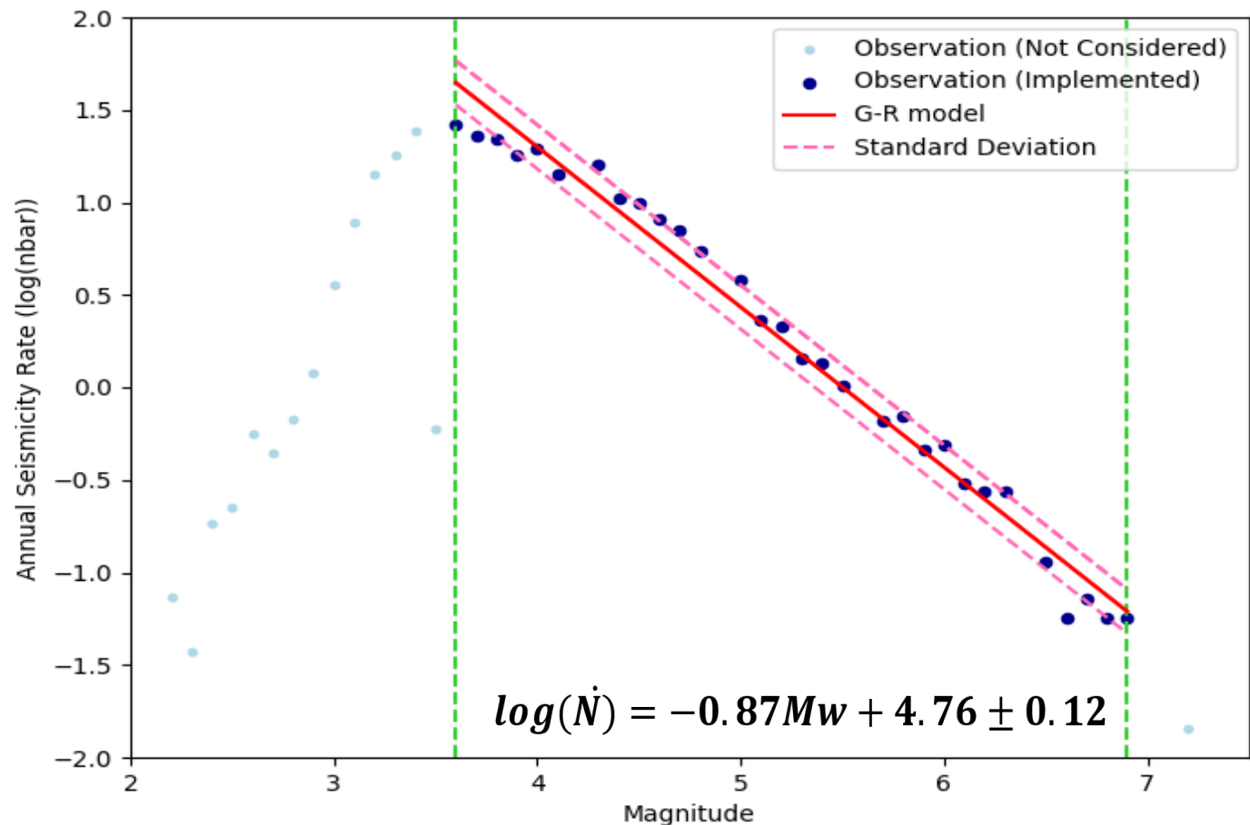
Magnitude–frequency distribution used for b-value estimation in the whole study area (Uhrhammer, 1986)
