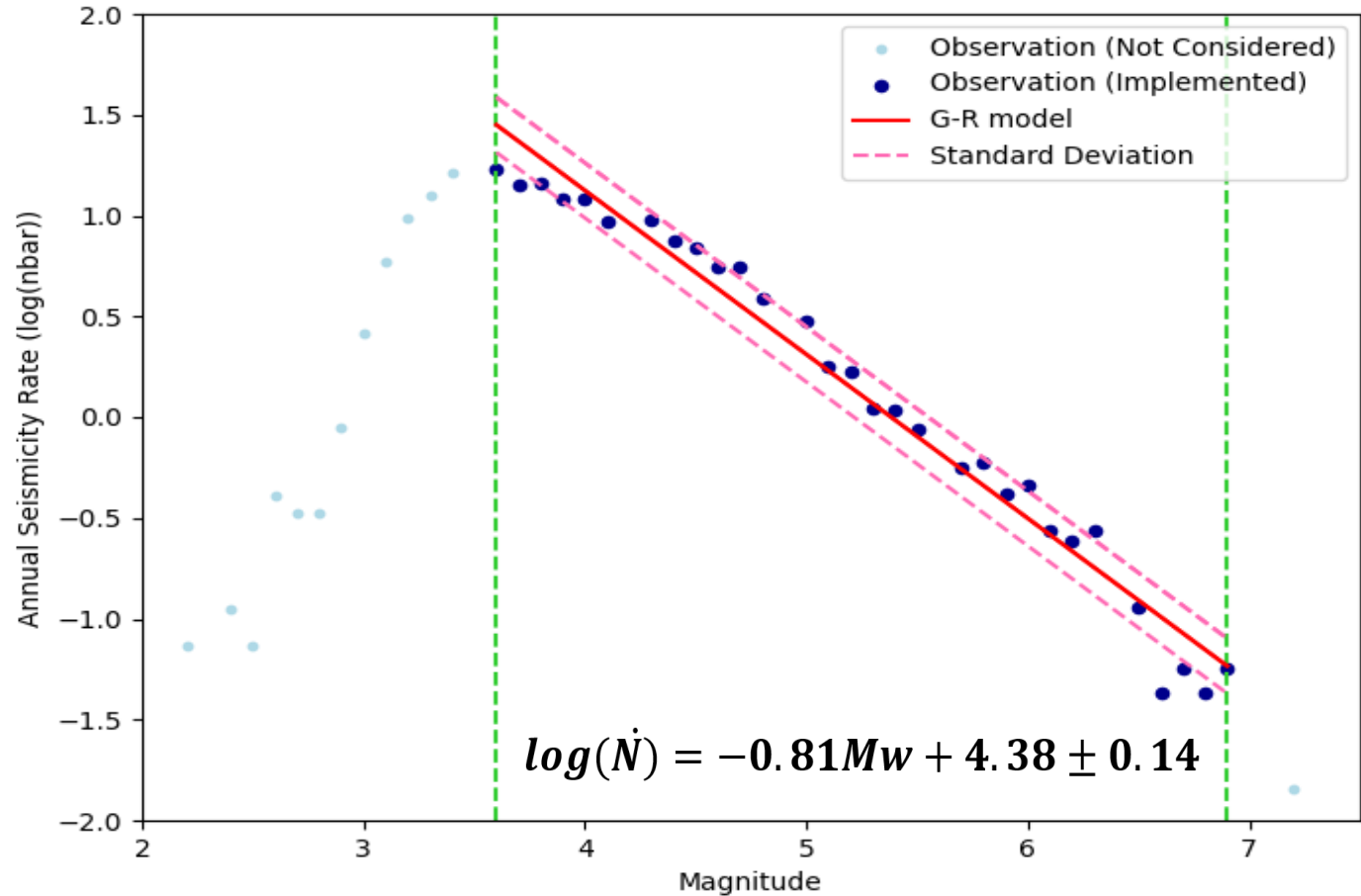
Magnitude–frequency distribution used for b-value estimation in the whole study area (Grünthal pers. comm.)
