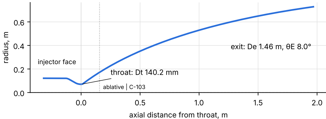
Thrust-chamber contour, Rao bell ( \theta_N 37.0^\circ , \varepsilon 108 , 80 %)
