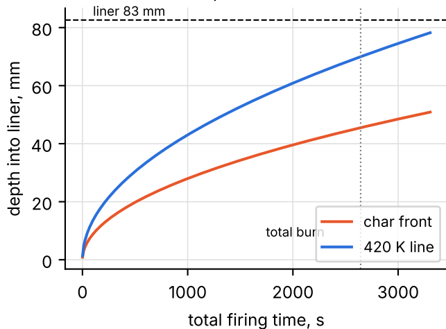
How deep the heat soaks in
