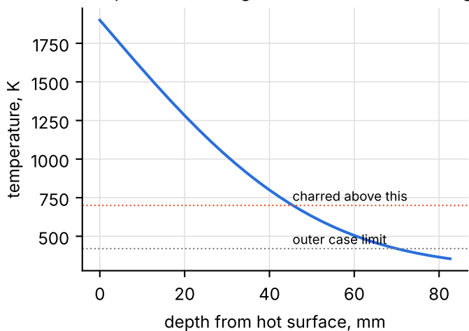
Temperature through the liner at end of firing
