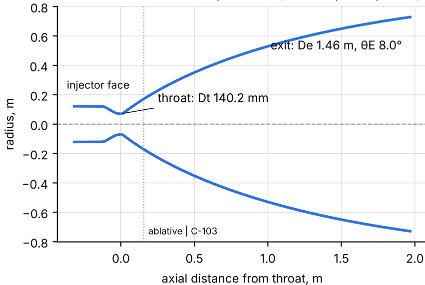
Thrust-chamber contour, Rao bell ( \theta_N 37.0°, \varepsilon 108, 80 %)
