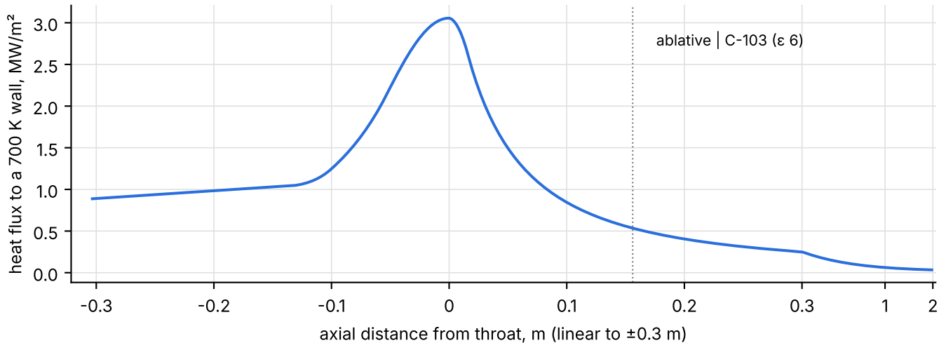
Gas-side heat flux along the engine
