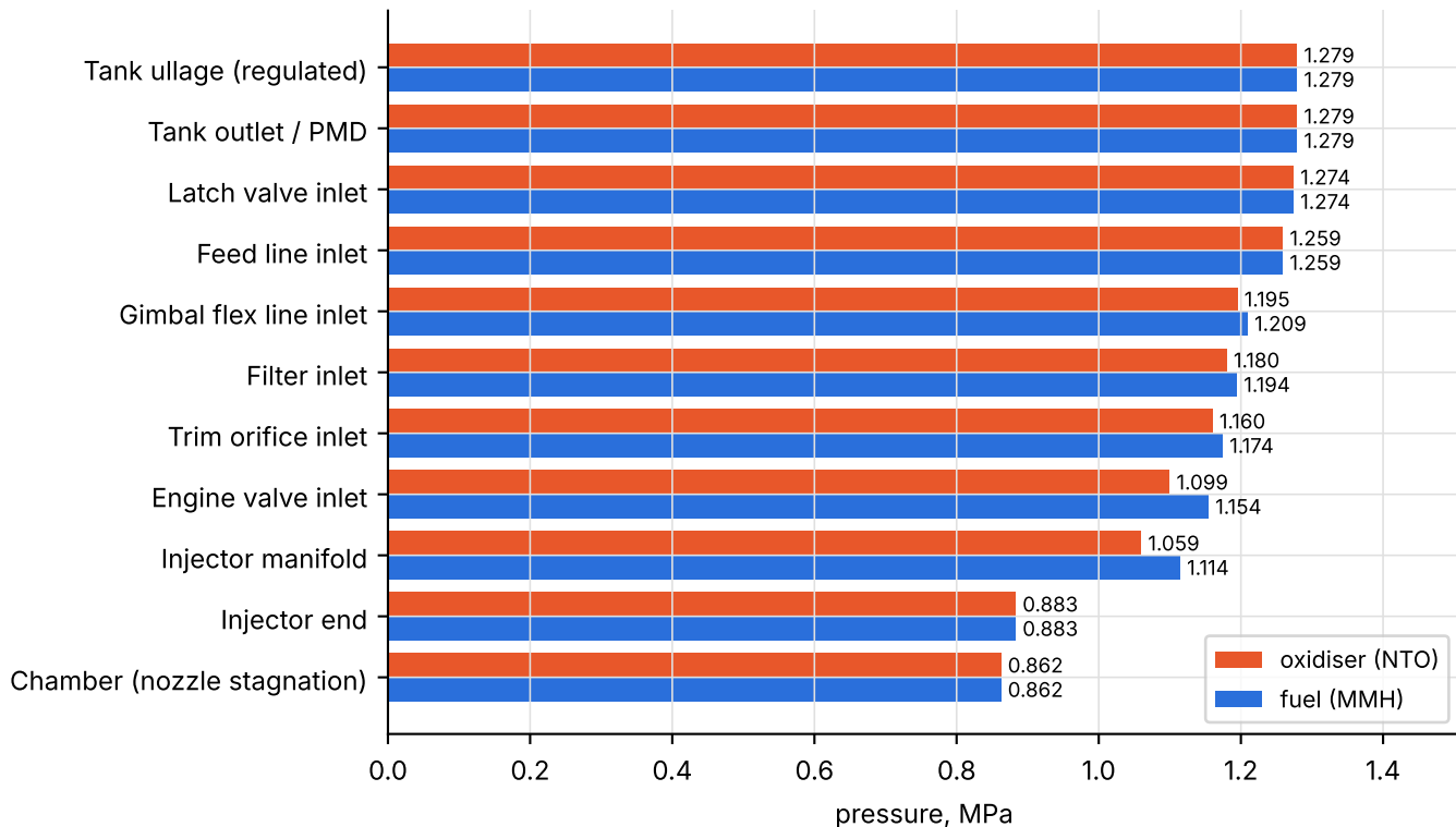
Pressure ladder (He regulator outlet 1.33 MPa; bottle 31 → 2.33 MPa)
