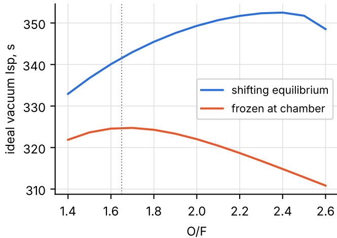
Ideal Isp vs O/F
