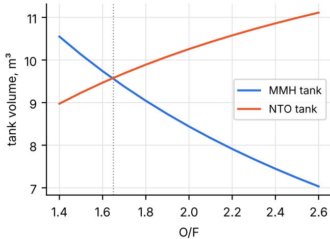
Tank volumes (sheet densities)
