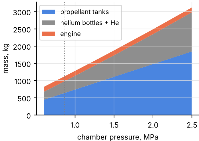
Propulsion-system mass
