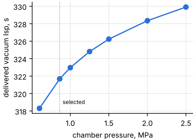
Isp (area ratio set by engine length)
