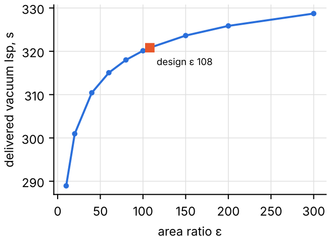
Vacuum Isp vs area ratio
