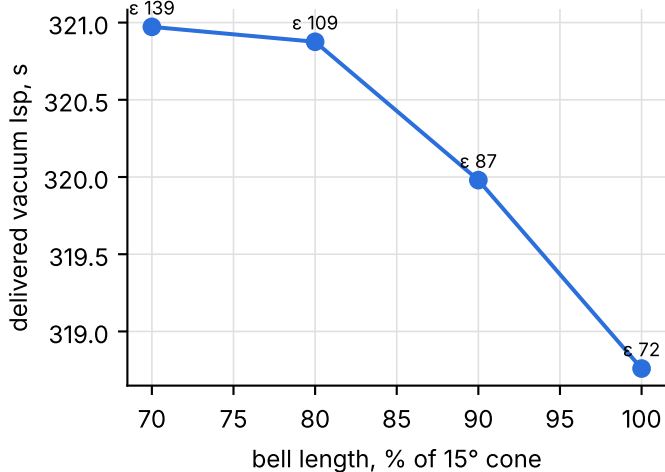
Same engine length, different bell length
