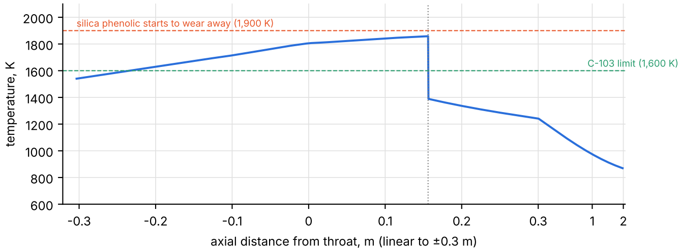
Hot-wall temperature: ablative chamber and throat, C-103 extension
