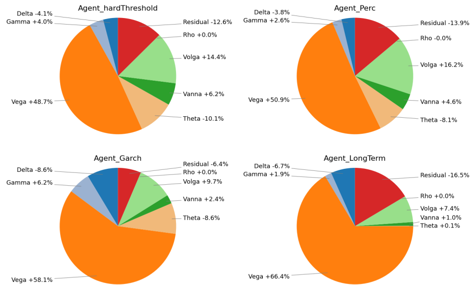
Figure 11: DIA Greeks diagnostics.
