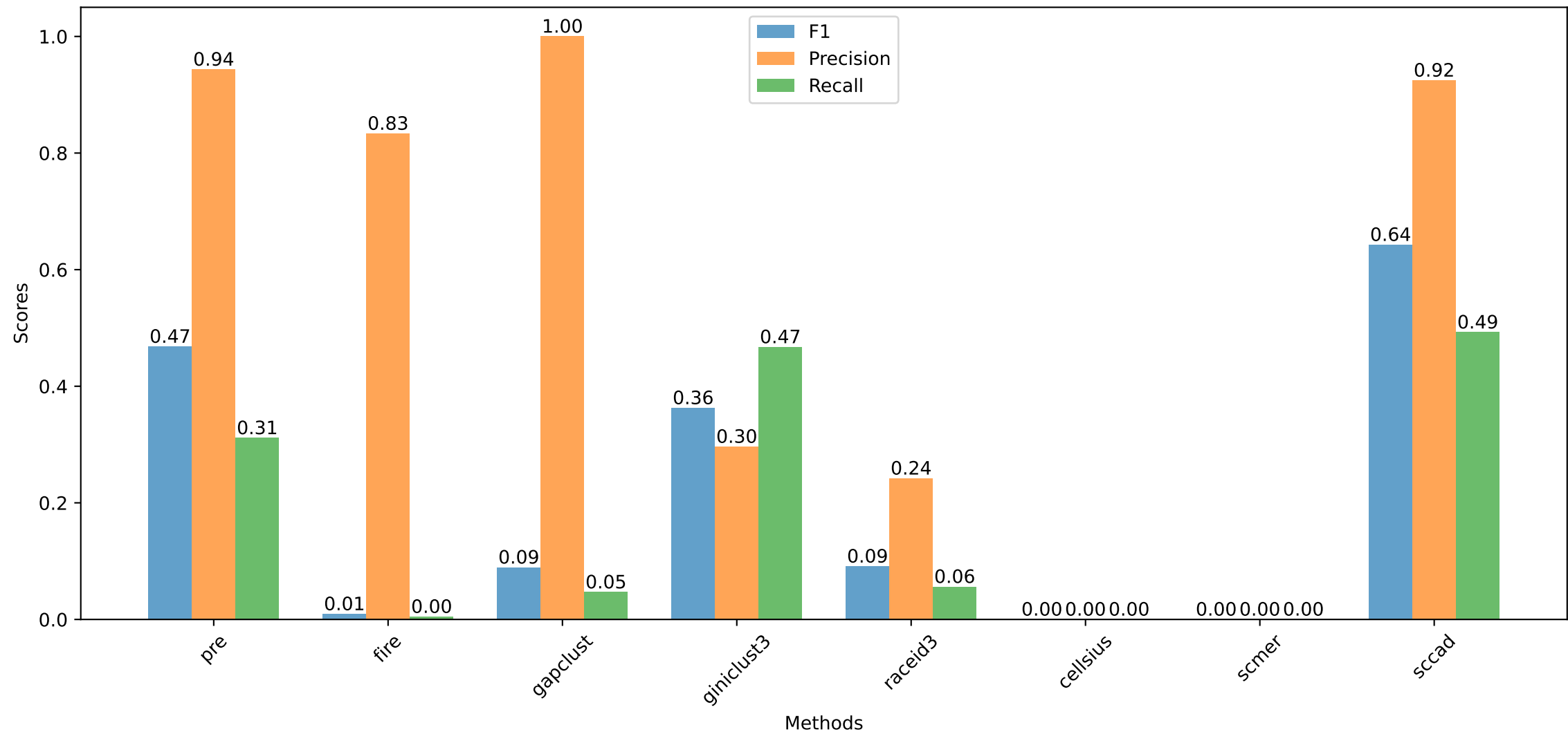
Performance Metrics for Rare Cell Prediction (<5%)
