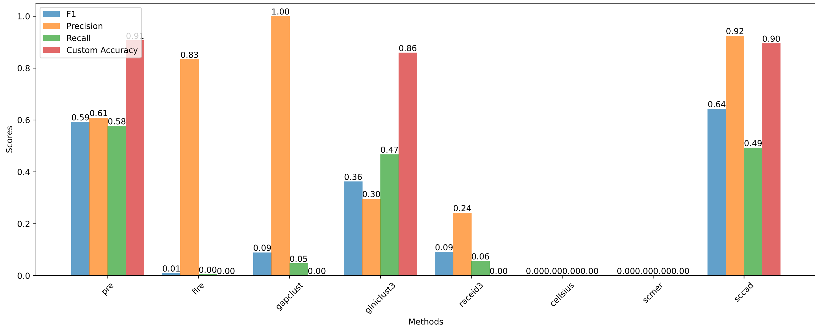
Performance Metrics for Rare Cell Prediction (&lt;5%)
