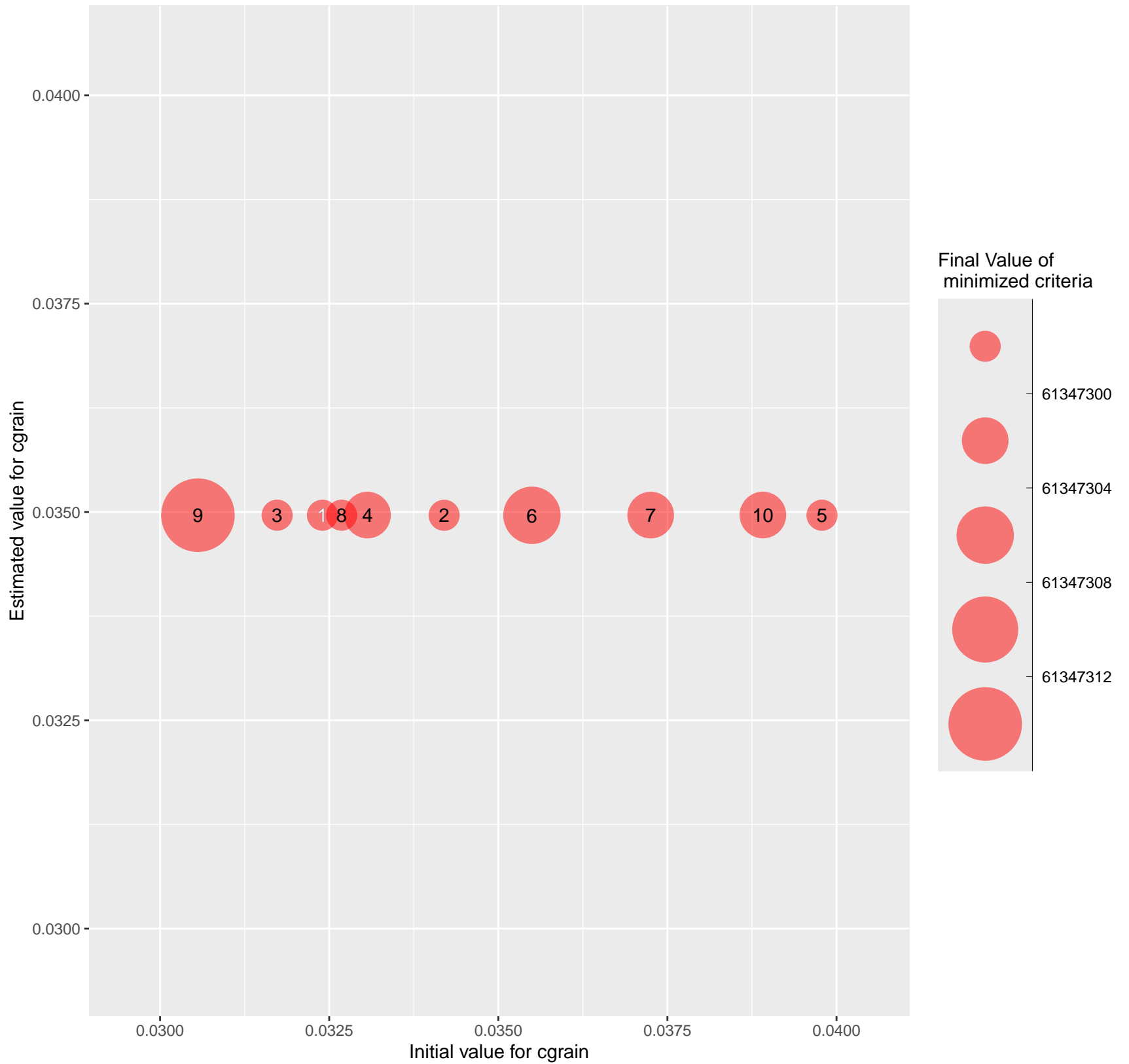
Estimated vs Initial values of cgrain for the different repetitions
