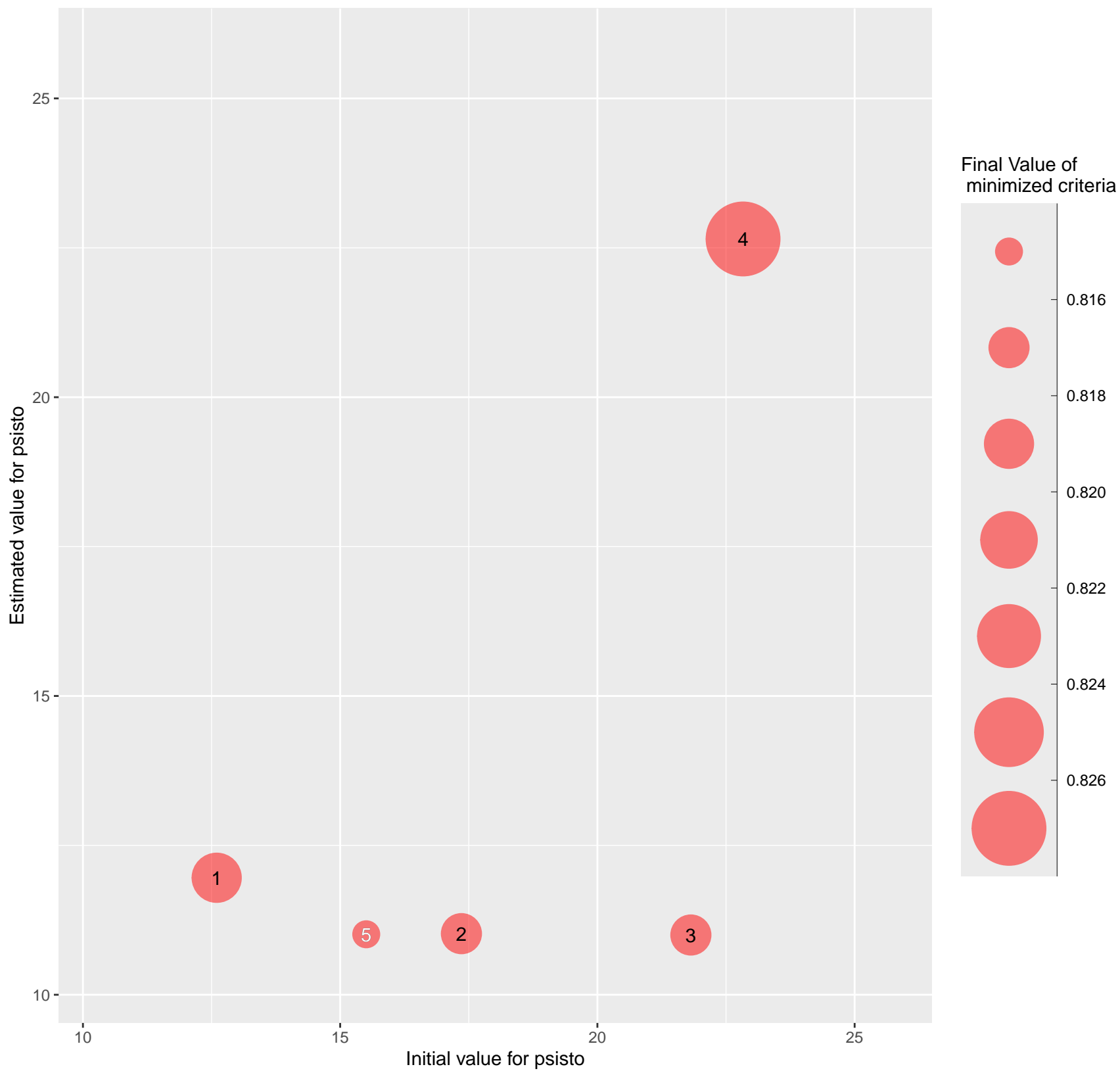
Estimated vs Initial values of psisto for the different repetitions
