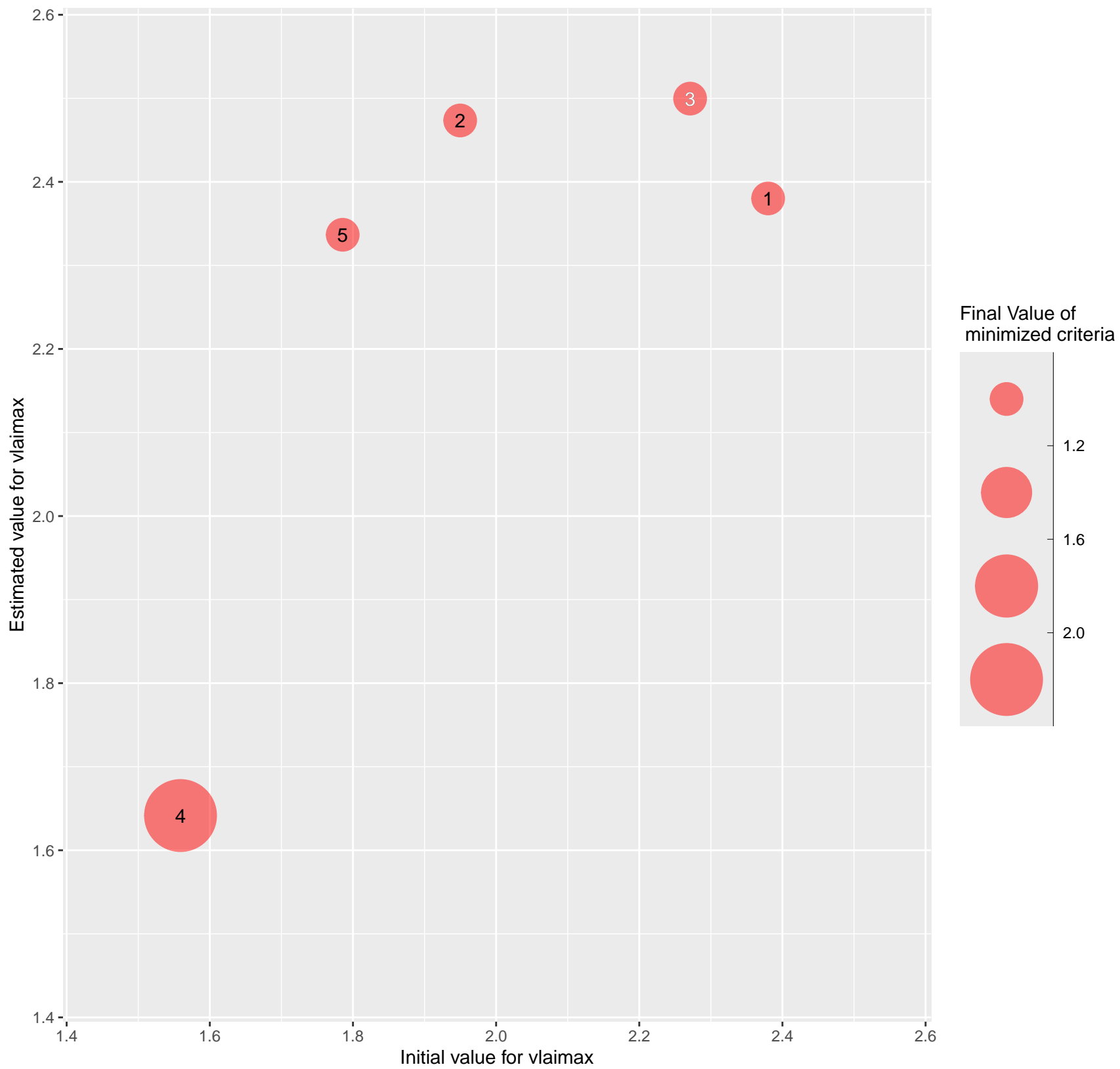
Estimated vs Initial values of vlaimax for the different repetitions
