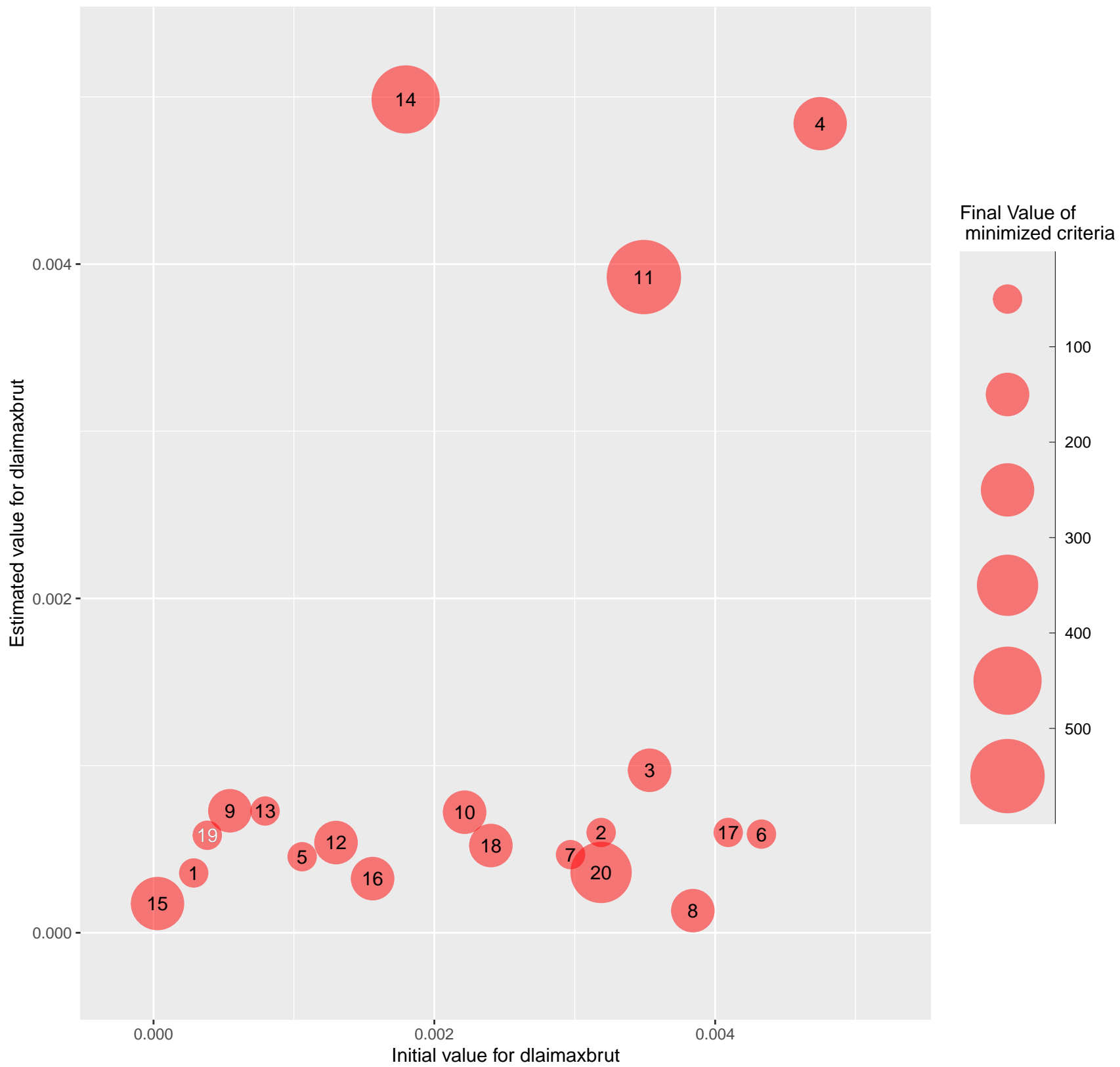
Estimated vs Initial values of dclaimxbrut for the different repetitions
