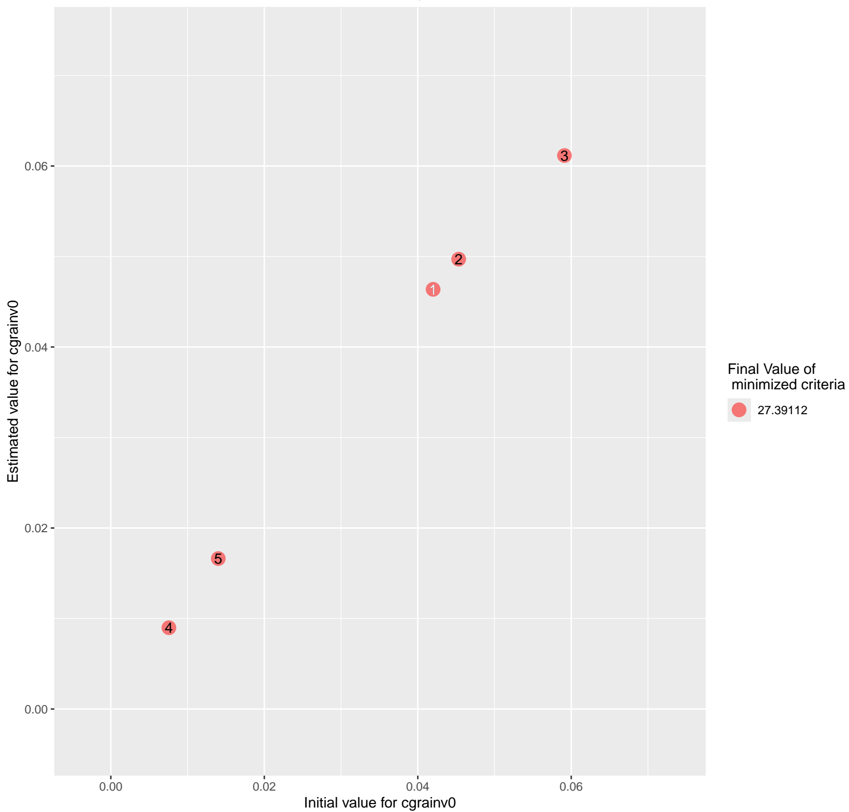
Estimated vs Initial values of cgrainv0 for the different repetitions
