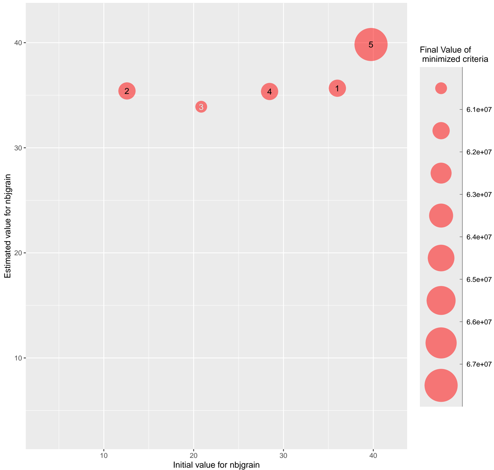
Estimated vs Initial values of nbjgrain for the different repetitions
