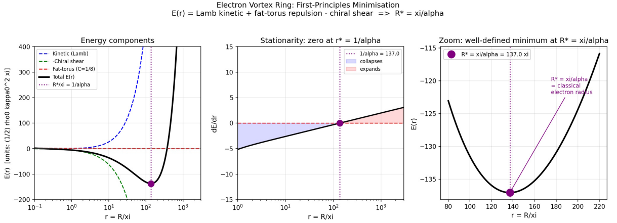
Figure 1: Electron vortex ring energy landscape. Left: The three contributions to \mathcal{E}(r) (17) in units of \frac{1}{2}\rho_0\kappa_0^2\xi : kinetic/Lamb (blue dashed), chiral-shear resistance (green dashed, negated), and fat-torus repulsion 2C/r (red dashed), with total \mathcal{E} (black). Centre: The stationarity condition d\mathcal{E}/dr changes sign exactly at r^* = 1/\alpha = 137 . Right: Zoom near the minimum confirming a well-defined bound state at R_e^* = \xi/\alpha = a_0/\sqrt{2} , not at the classical electron radius. Computed with \alpha = 1/137.036 .
