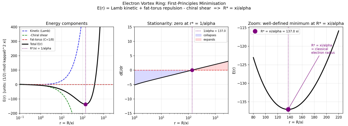
Figure 1: Electron vortex ring energy landscape. Left : The three contributions to \mathcal{E}(r) (??) in units of \frac{1}{2} \rho_0 \kappa_0^2 \xi : kinetic/Lamb (blue dashed), chiral-shear resistance (green dashed, negated), and fat-torus repulsion 2C/r (red dashed), with total \mathcal{E} (black). Centre : The stationarity condition d\mathcal{E}/dr changes sign exactly at r^* = 1/\alpha = 137 . Right : Zoom near the minimum confirming a well-defined bound state at R_e^* = \xi/\alpha (the classical electron radius). Computed with \alpha = 1/137.036 .
