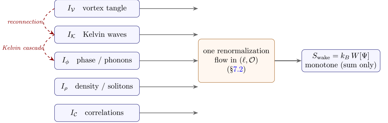
Figure 1: The wake architecture of W[\Psi] . Five physical channels (§5.3, calibrated in §6) carry the medium’s record of events. Dashed red arrows: inter-channel conversion at events — reconnection converts organized tangle into Kelvin and phonon content, and the Kelvin cascade decays into phonons (Table 1) — so individual channels are not monotone; only the sum is. All five enter a single coarse-graining flow in (\ell, \mathcal{O}) (§7.2), whose output is the wake entropy.
