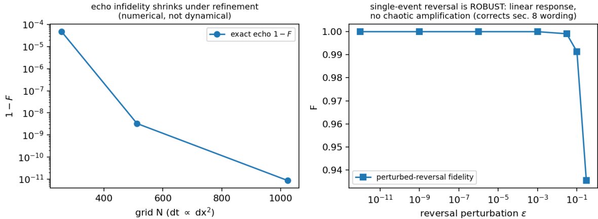
Figure 2: The #137 reversal-echo battery (script reversal_echo ; receipt in the result note). Left : exact-echo infidelity 1 - F through the annihilation event collapses under grid/timestep refinement ( 4.7 \times 10^{-5} \rightarrow 3.3 \times 10^{-9} \rightarrow 8.7 \times 10^{-12} at N = 256/512/1024 , dt \propto dx^2 ) — the losses are numerical (dealiasing projection and round-off), not dynamical: the dynamics is conservative, and branch B is dead as written. Right : fidelity of the \varepsilon -perturbed reversal: flat at the exact-echo plateau from \varepsilon = 10^{-12} through 10^{-3} and equal to the forward-propagation overlaps at the same \varepsilon (linear response, no chaotic amplification) — the measured correction to this section’s earlier “exquisitely tuned boundary data” wording: single-event reversal is robust, and the arrow rests on scale, multiplicity, and the absence of any natural conjugation operation.
