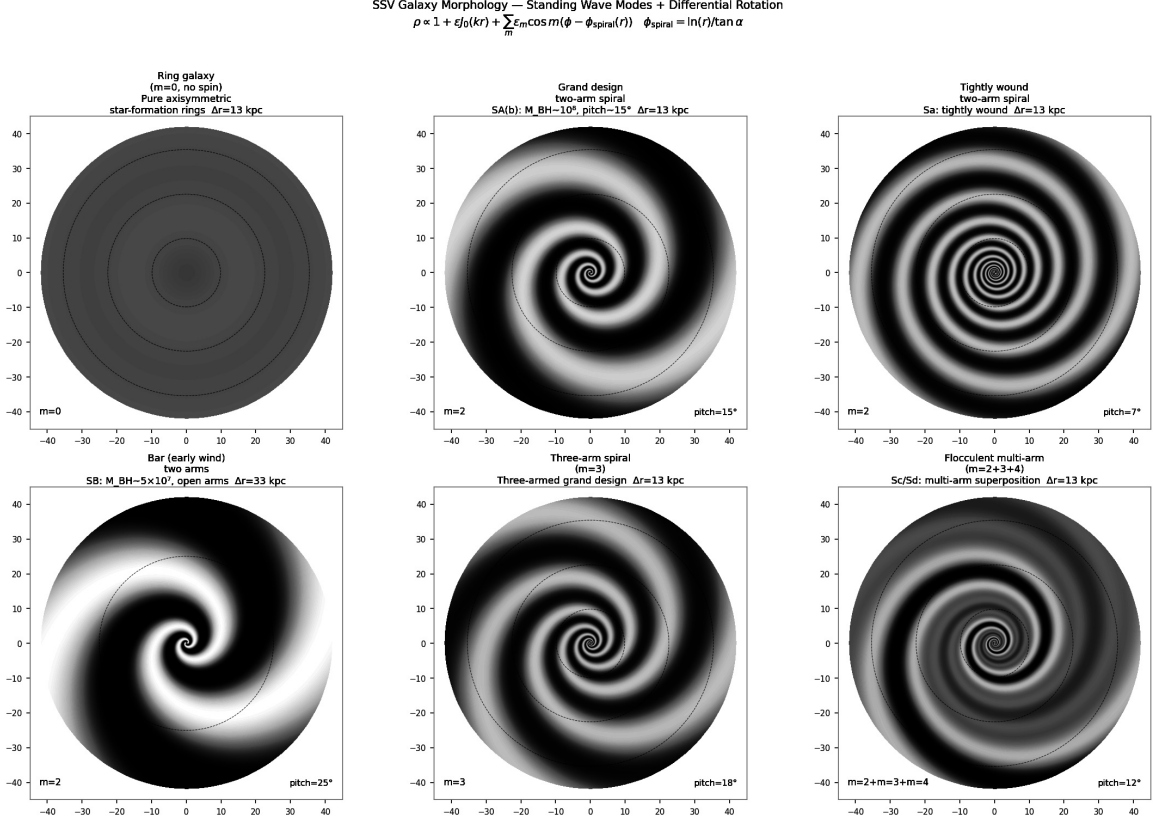
Figure 3: The SSV morphology zoo from equation (1) with differential rotation applied. Top row : ring ( m = 0 , no spin); grand-design two-arm ( m = 2 , pitch 15°); tightly wound Sa ( m = 2 , pitch 7°). Bottom row : bar + two arms ( m = 2 , large pitch, small M_{\text{BH}} ); three-arm ( m = 3 , pitch 18°); flocculent multi-arm ( m = 2 + 3 + 4 , pitch 12°). All cases use \mathcal{C} = 1.8 \times 10^9 \text{ kpc} \cdot M_{\odot} . No dark matter; no free structural parameters.
