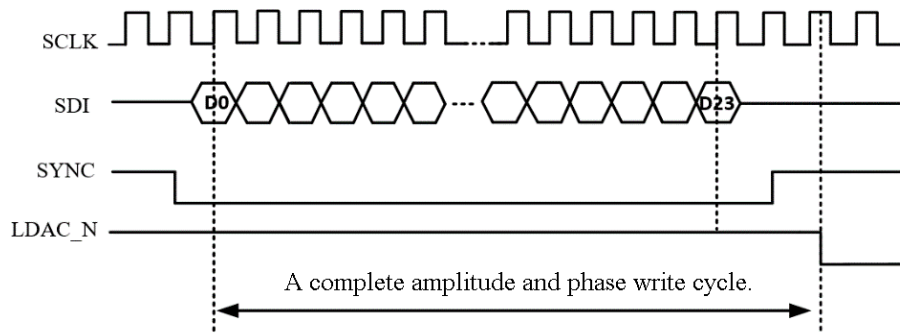
Figure 25. SPI Write Timing
