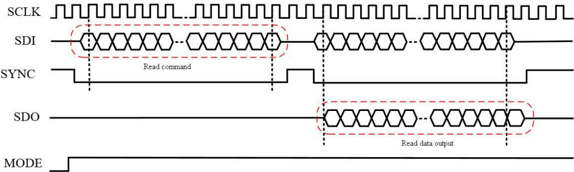
Figure 26. SPI Read Timing
