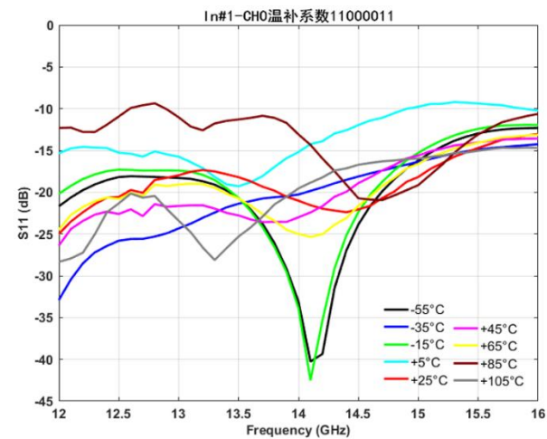
Figure 18. Input Echo Variations under High and Low Temperatures (-55°C - +105°C)
