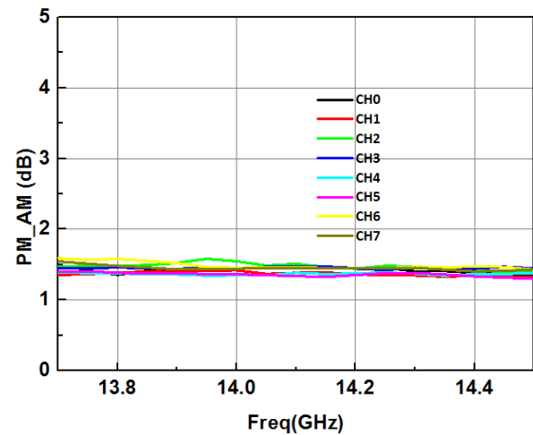
Figure 14. Parasitic Amplitude Modulation of Phase Shift
