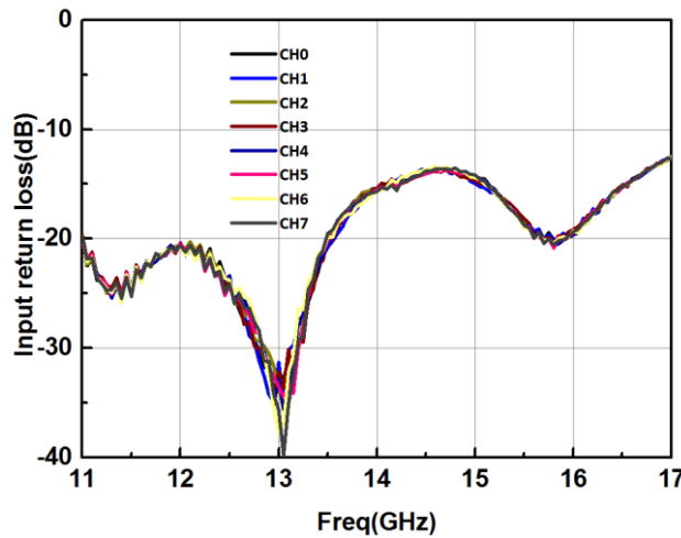
Figure 5. Relationship between Return Loss and Frequency with Different Channels
