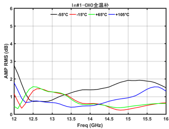
Figure 21. Amplitude Modulation Variations under High and Low Temperatures (-55°C - +105°C)
