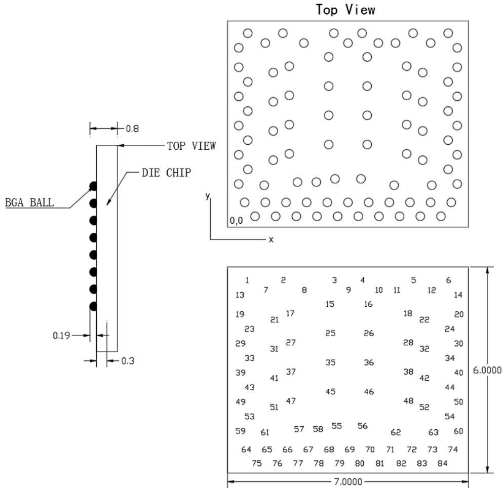
Figure 2. Pin Configuration Diagram
