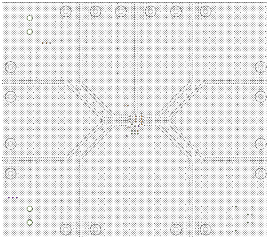
Fig. 33. L2 Layer of Multifunctional Integrated Chip Evaluation Board
