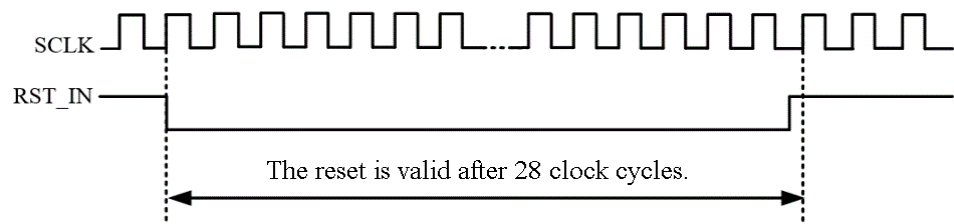
Figure 23. SPI Reset Timing
