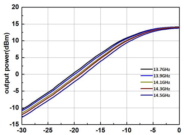
Figure 7. Relationship between Single-Channel Output Power and Input Power
