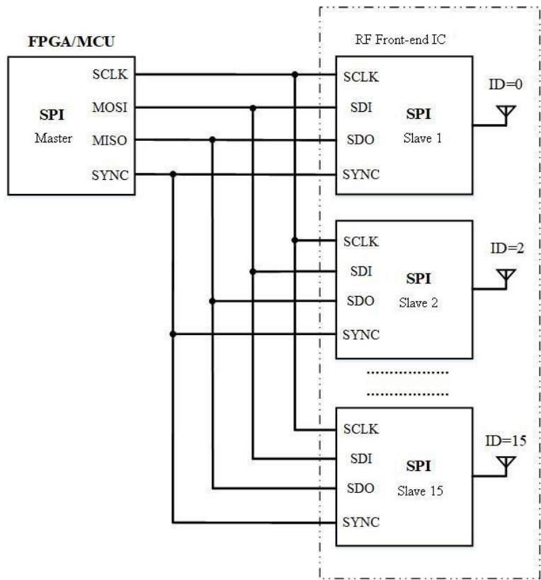
Figure 24. SPI Hardware Topology Diagram
