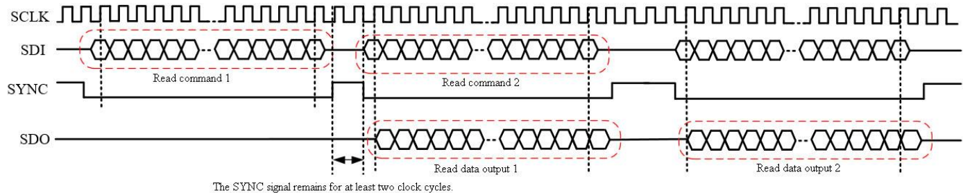
Figure 27. SPI Pipeline Schematic
