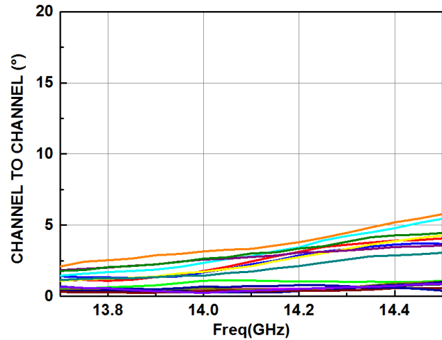
Figure 16. Phase Position Influence between Different Channels
