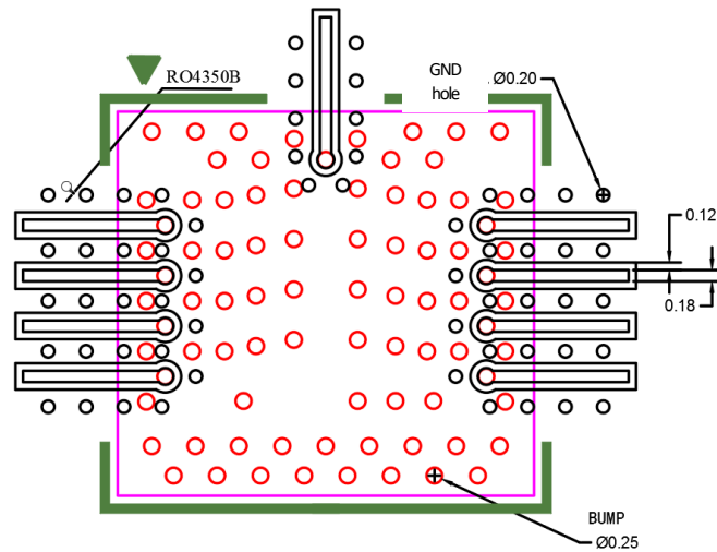
Figure 28. Recommended Application of RF SMT
