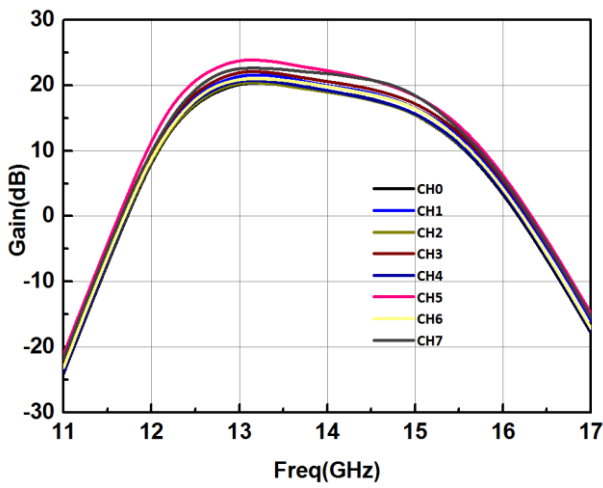
Figure 4. Relationship between Gain and Frequency with Different Channels
