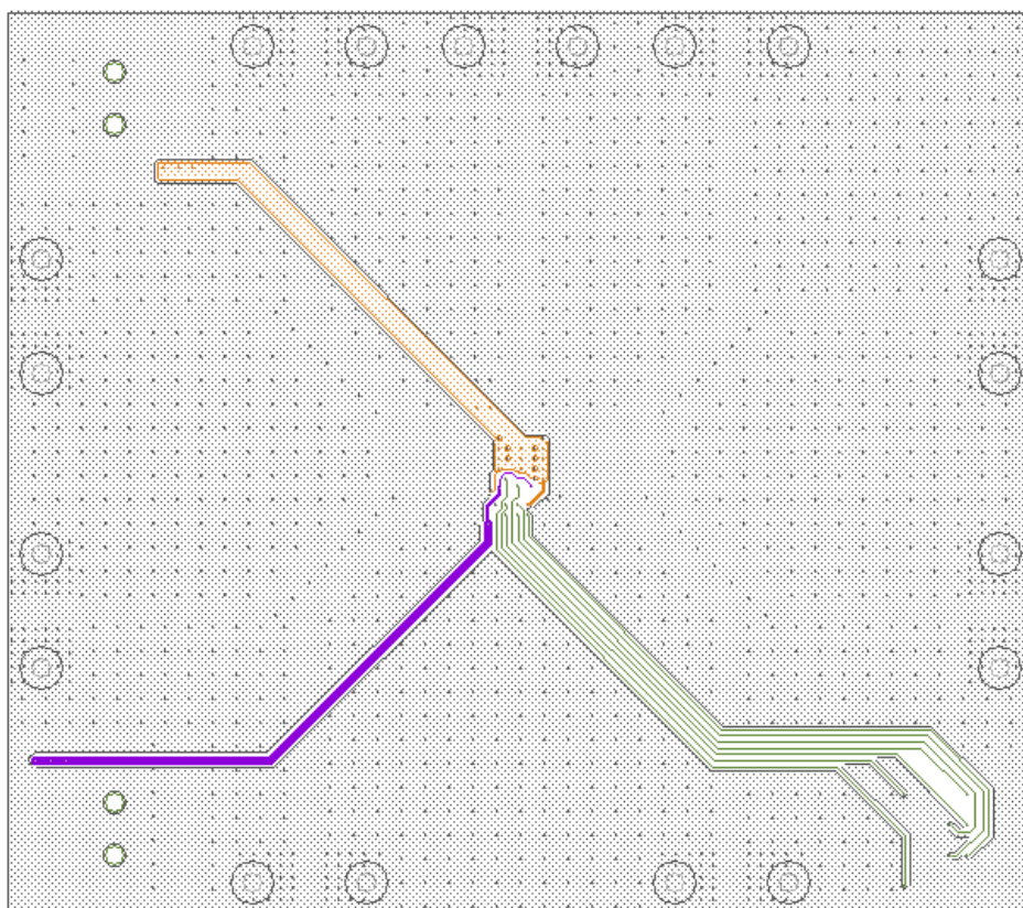
Figure 34. L3 Layer of Multifunctional Integrated Chip Evaluation Board
