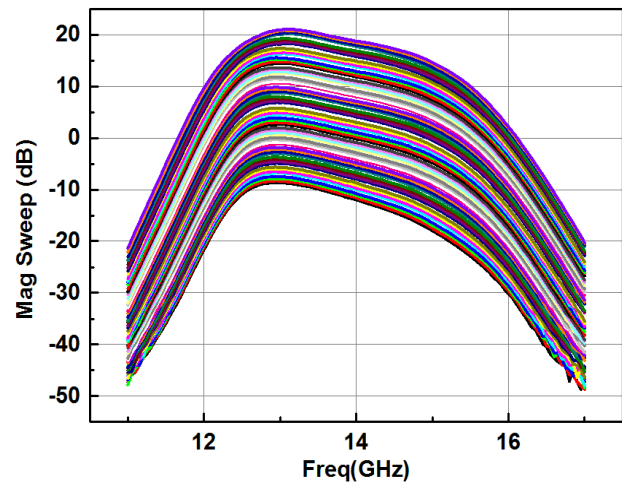
Figure 10. Amplitude Modulation (64-state)
