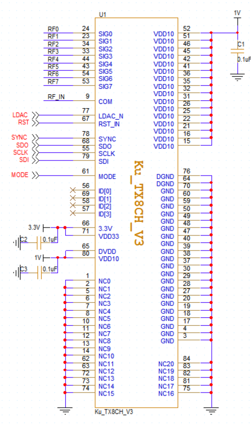
Figure 31. Schematic Diagram of Multifunctional Integrated Chip Evaluation Board
