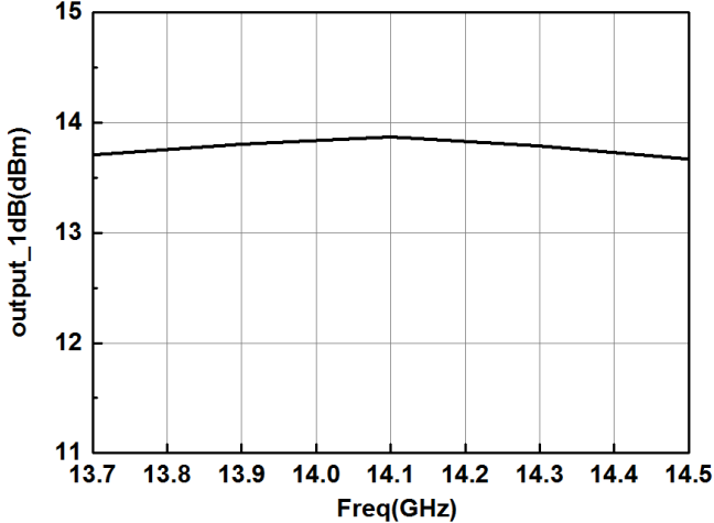
Figure 8. Output Power of the Single Channel (p-1dB)
