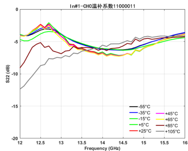
Figure 19. Output Echo Variations under High and Low Temperatures (-55°C - +105°C)
