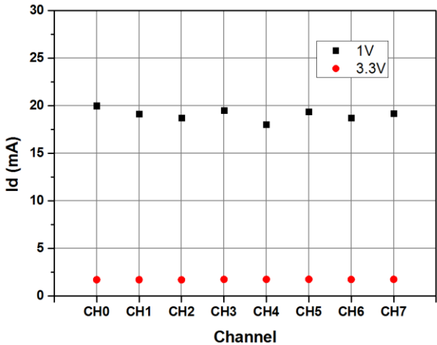
Figure 3. Operating Current under Single-Channel Status
