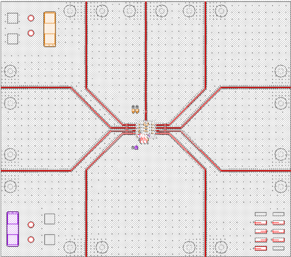
Fig. 32. Top Layer of Multifunctional Integrated Chip Evaluation Board
