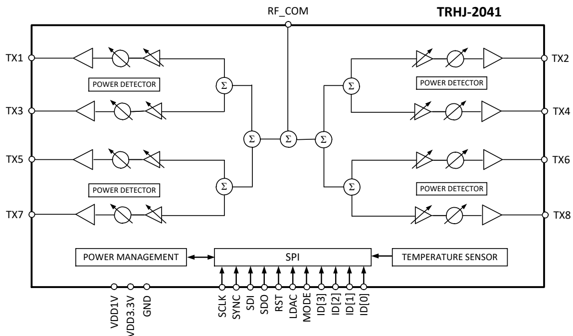
Figure 1 Functional Block Diagram of Chip
