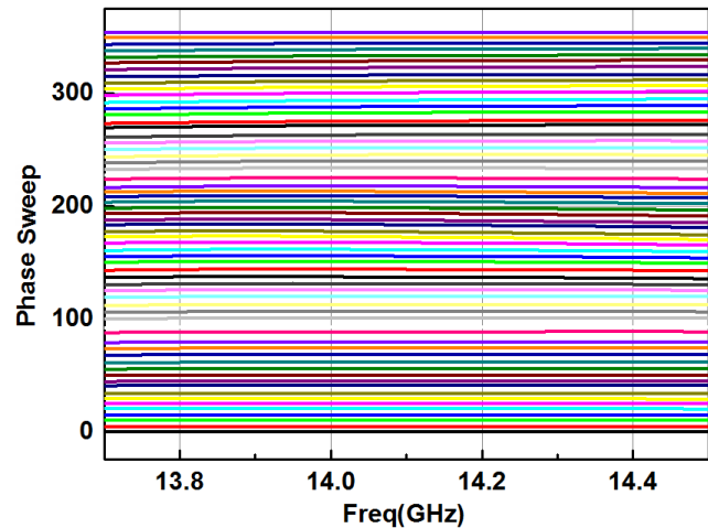
Figure 12. Relationship between 64 Phase Shift States and Frequency
