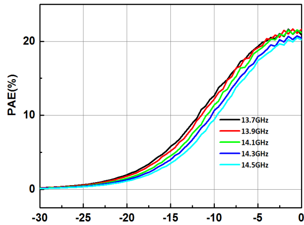
Figure 9. Relationship between Single-Channel Output Power and Efficiency
