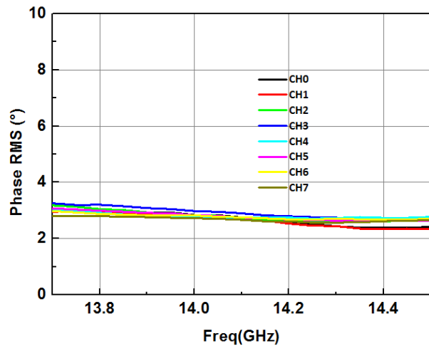
Figure 13. Relationship between 8 Channel Phase Shift RMS and Frequency
