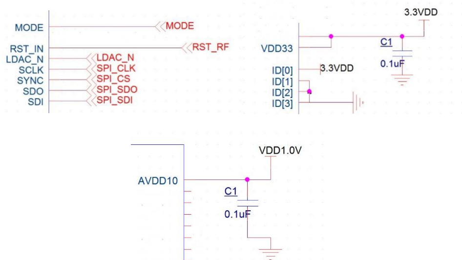
Figure 29. Recommended Peripheral Bias of Multifunctional Integrated Chip
