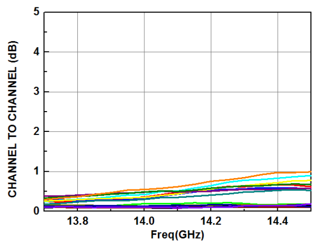
Figure 15. Amplitude Influence between Different Channels
