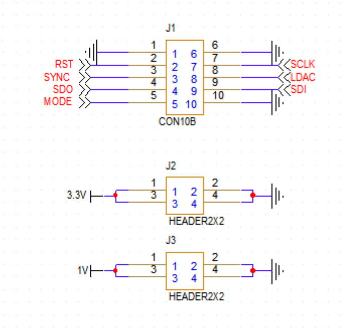
Figure 30. Schematic Diagram of Multifunctional Integrated Chip Evaluation Board
