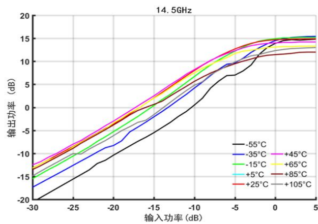
Figure22. Output Power Variations under High and Low Temperatures (-55°C - +105°C)
