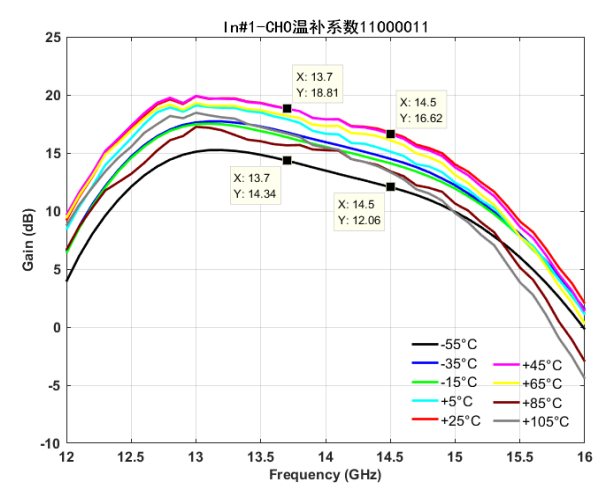
Figure 17. Gain Variations under High and Low Temperatures (-55°C - +105°C)
