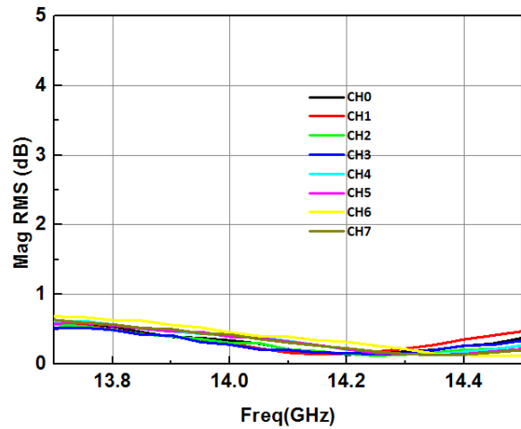
Figure 11. Relationship between 8 Channel Amplitude RMS and Frequency
