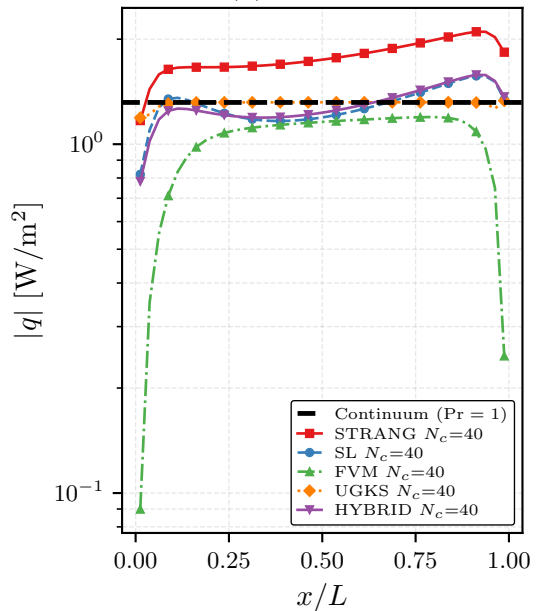
(c) Heat flux
