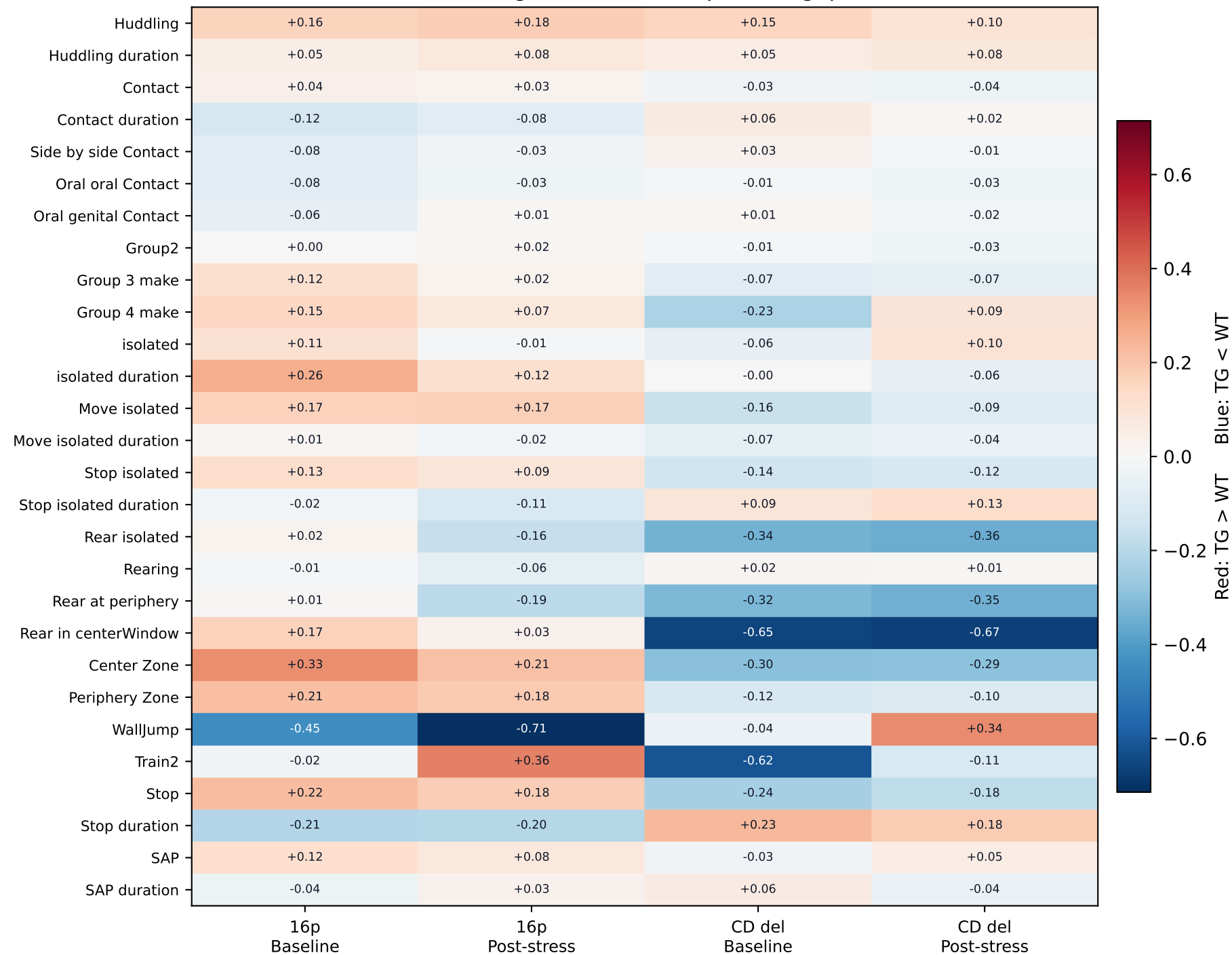
Behavioral signature: TG - WT paired log1p deltas
