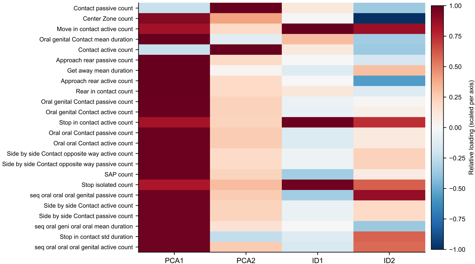
Feature loadings on the projection axes
