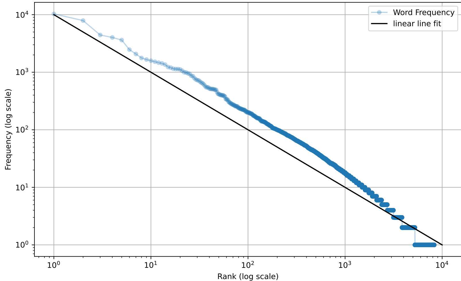
Word Frequency as a Function of Word Rank (Zipf's Law)
