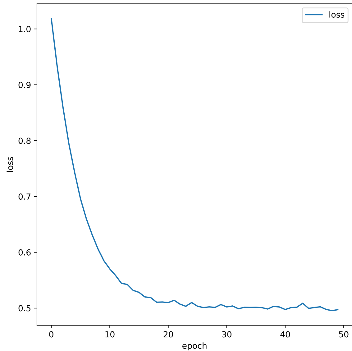
Loss over iterations
