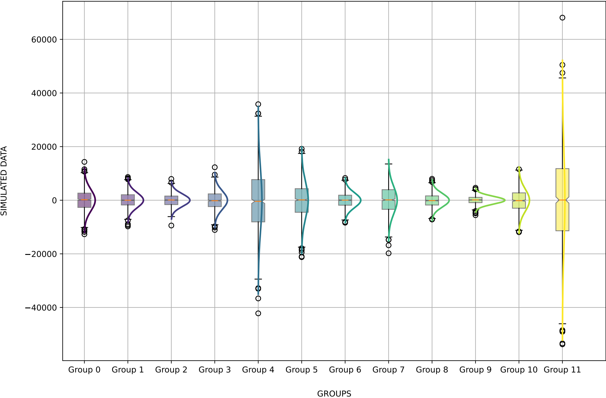
Boxplots / Estimated Distribution for Each Group with Notches Showing 95% Confidence Intervals
