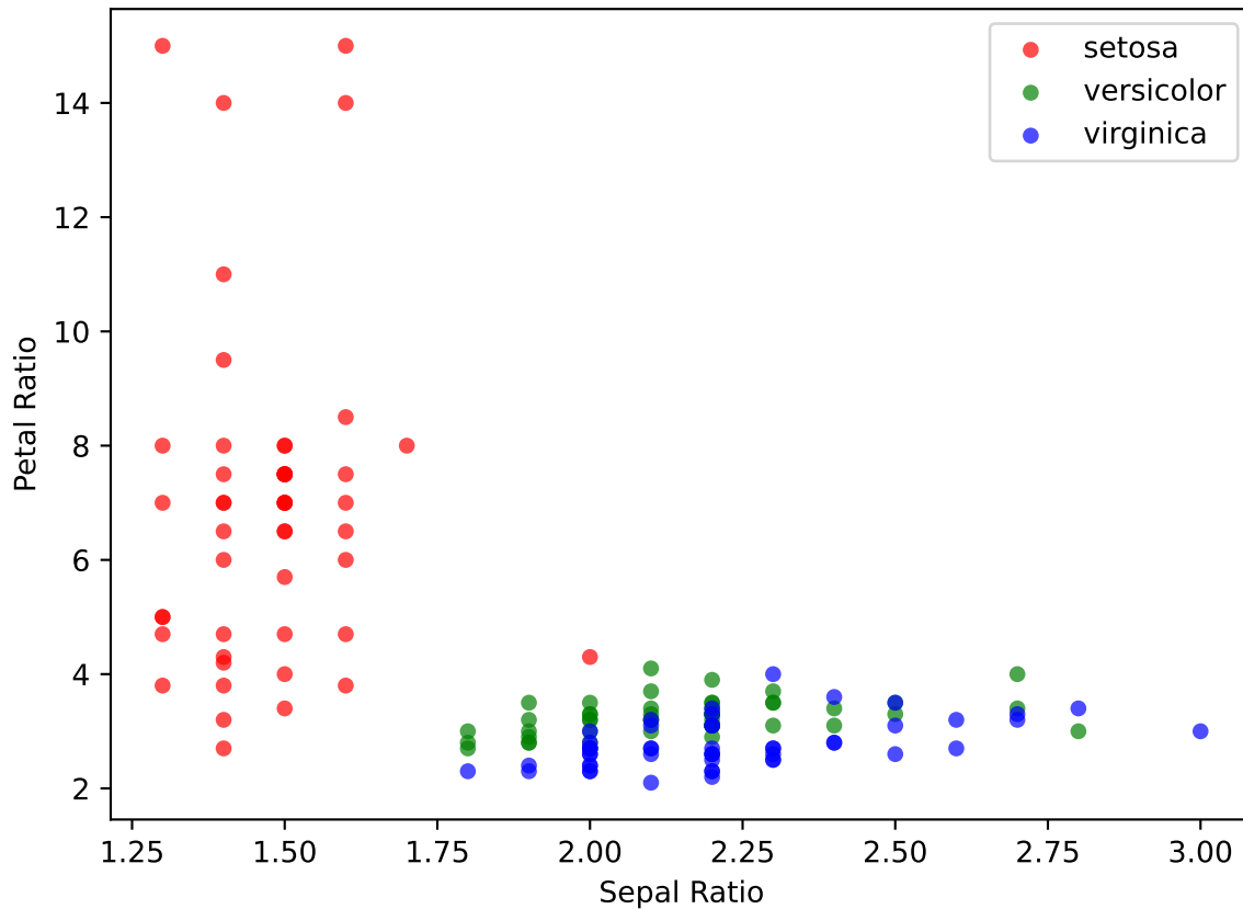
Scatter plot of Sepal Ratio vs Petal Ratio for each species
