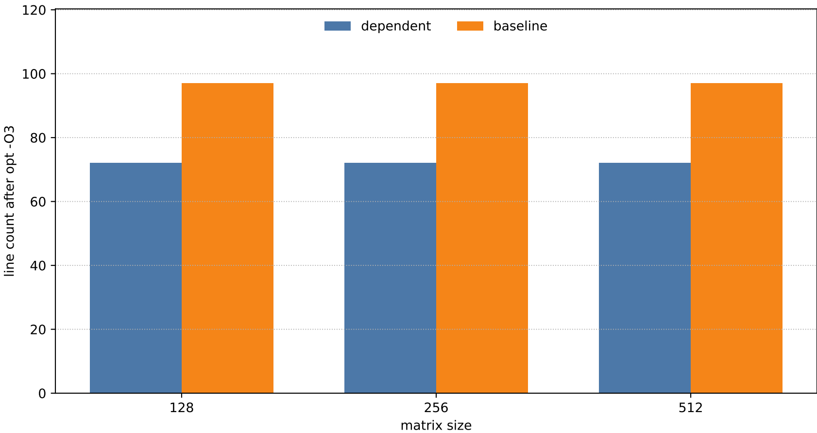
Optimized LLVM IR Line Count
