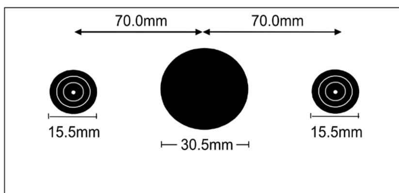
10m Moving Target Electronic Target The 30.5mm diameter is a hole.
