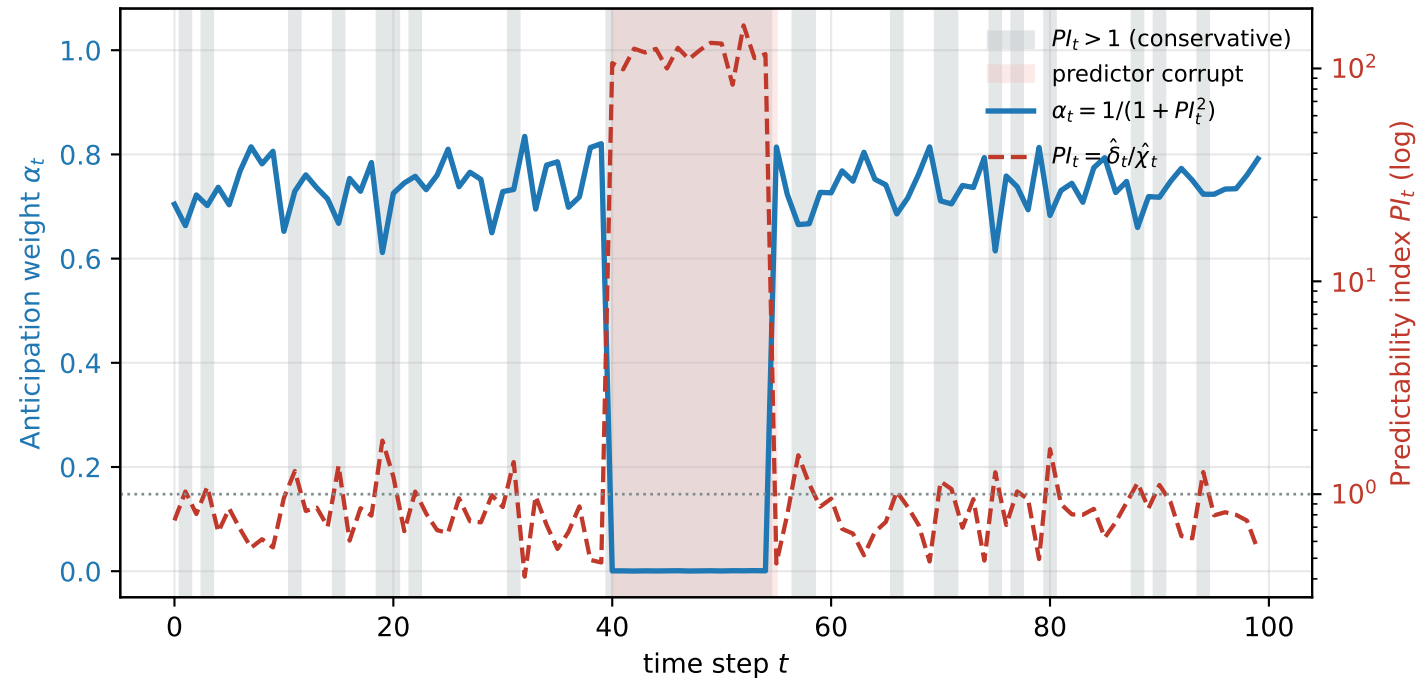
Thm.3 / PAP: continuous PI-conditioned interpolation (not hard switching)
