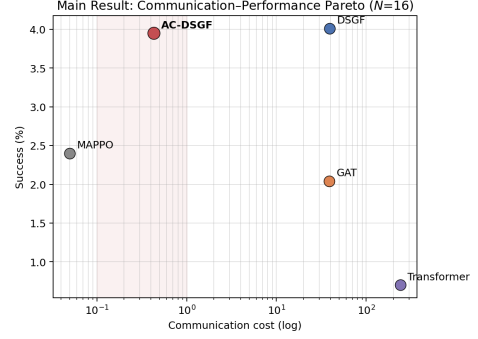
Fig. 8. Communication-performance Pareto ( N=16 , Table V). AC-DSGF occupies the high-efficiency region (left): comparable Success at minimal communication cost.
