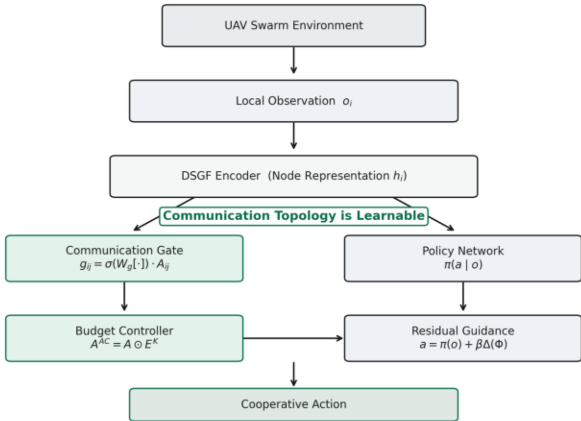
Fig.1 AC-DSGF Framework | Communication Topology is Learnable
