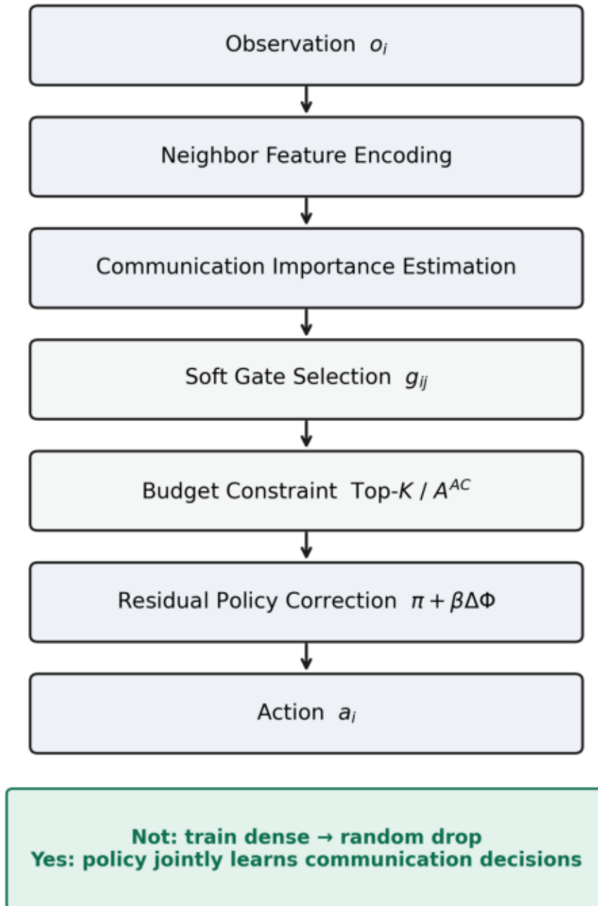
Fig.3 Algorithm Pipeline (joint policy-communication learning)
