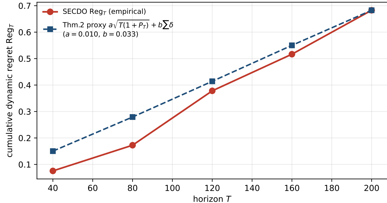
Theory validation: regret scales with \sqrt{T(1 + P_T)} (synthetic)
