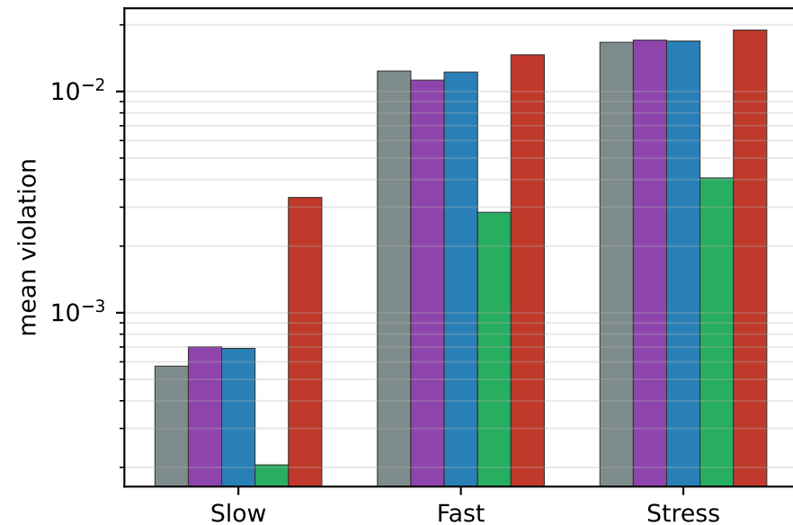
Constraint violation
