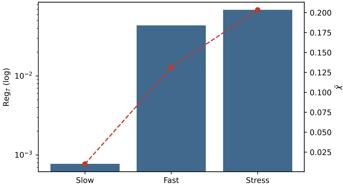
Verify: Regret vs Drift (from EVIDENCE_CHAIN)
