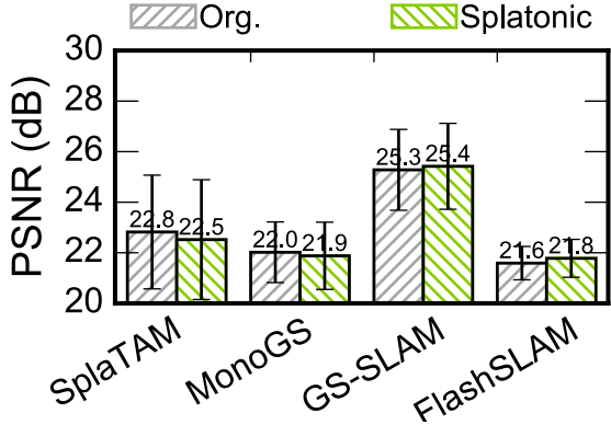
(b) Reconstruction quality. Higher is better.
