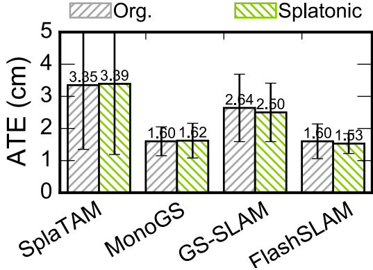
(a) Tracking accuracy. Lower is better.
