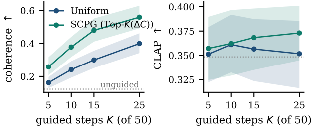
Fig. 2. Budget sweep on a paired 50-trial subset: coherence (left) and CLAP (right) against the number of guided steps, uniformly spread vs placed at the steps of highest steering sensitivity (mean, bootstrap 95% CI). Dotted: unguided.
