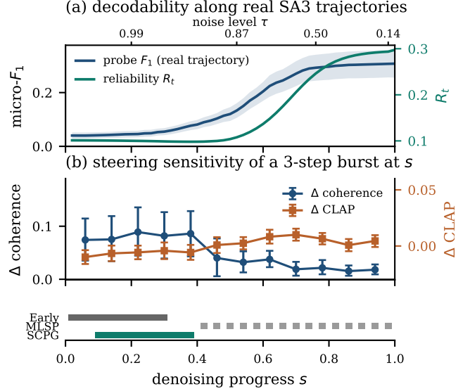
Fig. 3. The same analysis on Stable Audio 3 medium (base, 50 steps): (a) probe micro- F_1 and reliability R_t along 50 real development trajectories; (b) change in coherence and in CLAP from a three-step burst starting at one position (mean, 95% CI, 50 paired development trials). Top axis: noise level \tau at each position. Bottom: guided steps of the Early, MLSP-fixed and SCPG schedules on SA3.
