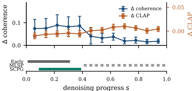
(b) steering sensitivity of a 3-step burst at s
