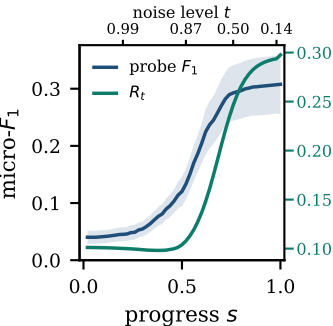
(a) decodability
