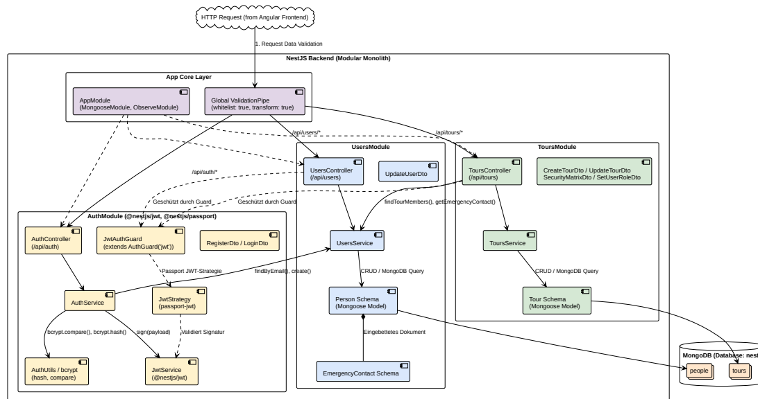
Figure 4: Bausteinsicht Level 2: NestJS Modular Monolith Struktur (PlantUML: 04_backend_architektur.puml)
