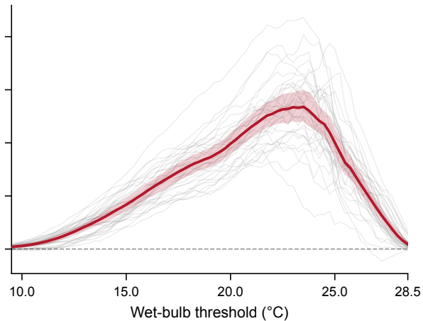
Largest connected exceedance area
