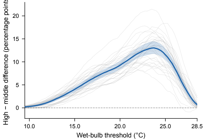
Simultaneous exceedance area
