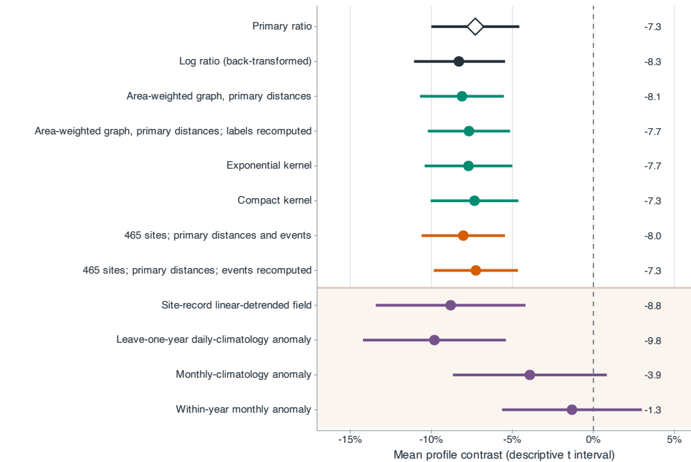
Figure 7 Robustness of the mean profile contrast. Dark rows denote the main and transformation analyses; green, orange and purple rows denote graph construction, spatial resolution and field definition. Points and bars are estimates and descriptive t -reference intervals based on between-summer variation. Alt text: A forest plot shows mostly overlapping negative estimates across transformation, graph and resolution choices. Two purple-shaded anomaly-field rows lie closest to zero.
