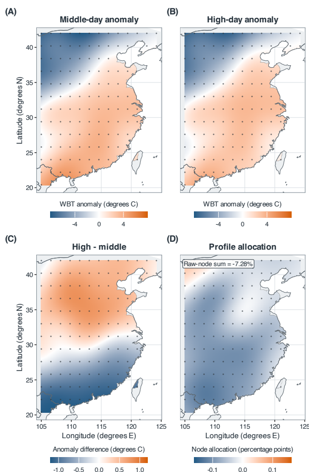
Figure 4 Spatial structure of the primary 121-site evaluation contrast. (A,B) Middle- and high-day within-field anomalies; (C) their difference; (D) exact observed-node allocations averaged over the five prespecified graph scales. The 121 allocations sum to -7.28\% , identical to the primary finite-record estimand. The interpolated surfaces visualise the 121 observed-node values; estimation and inference use the observed nodes.
