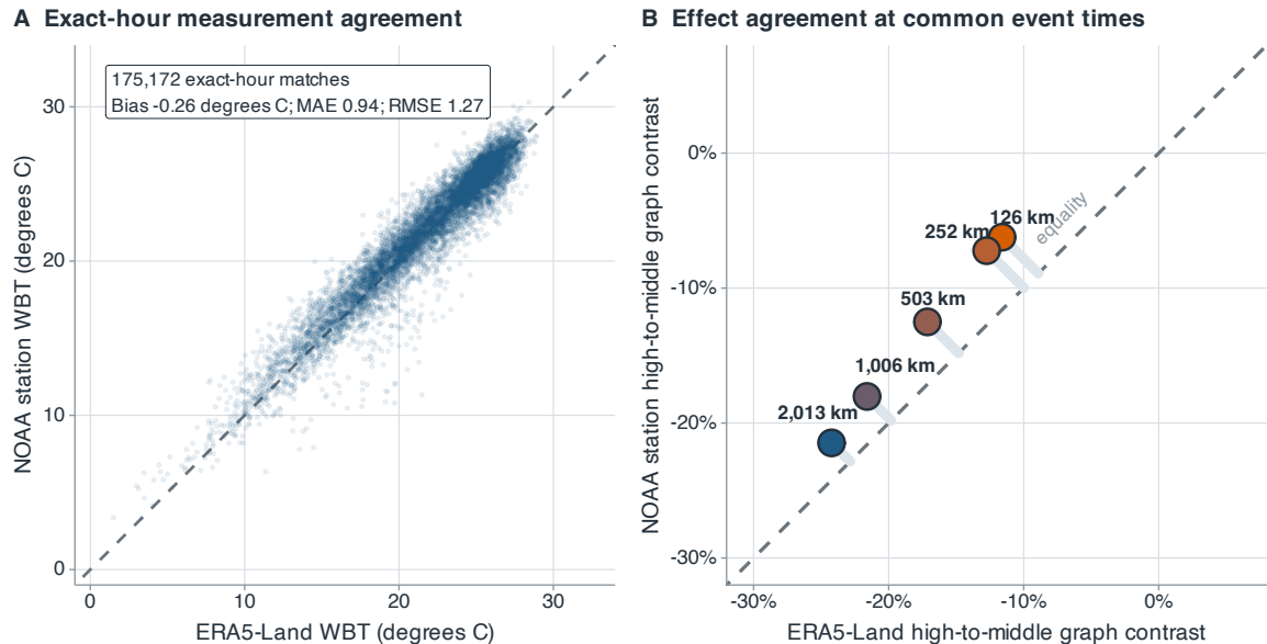
Figure 7 NOAA station and ERA5-Land agreement in ten summers excluded from method development. (A) Exact-hour WBT at 28 stations, with summaries from all 175,172 matches. (B) High-middle graph contrasts at the five fixed bandwidths, using ERA5-Land peak times and labels and identical station subsets. Dashed diagonals denote equality; pale segments in panel B connect station estimates to equality.
